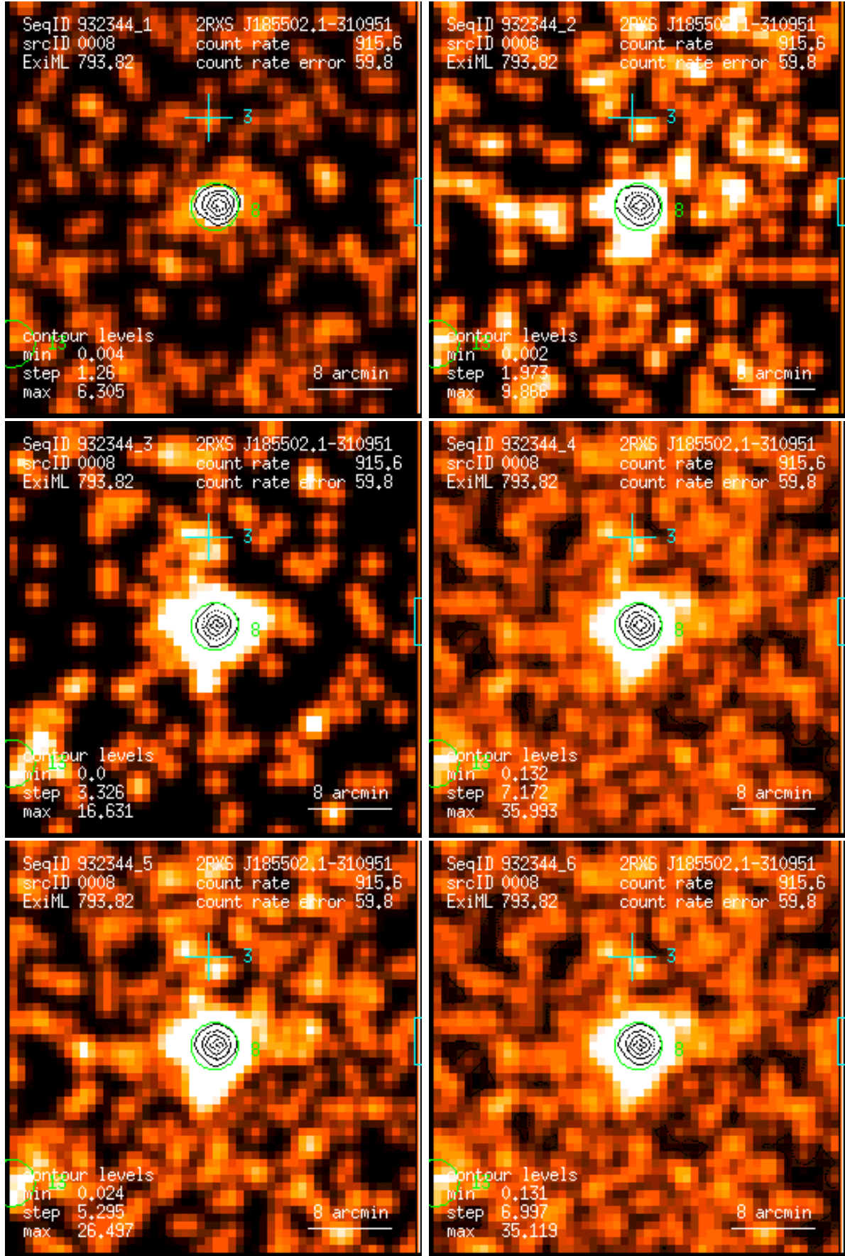
Figure 8: RASS 932344: detection 0008: band rate images, Gaussian filter: (1) PSPC channels 11 – 41, (2) 52 – 90, (3) 91 – 201, (4) 11 – 235, (5) 52 – 201, (6) 11 – 201. Broad band rates in counts/ks. Band rate contour levels in counts/ks/arcmin 2 .
