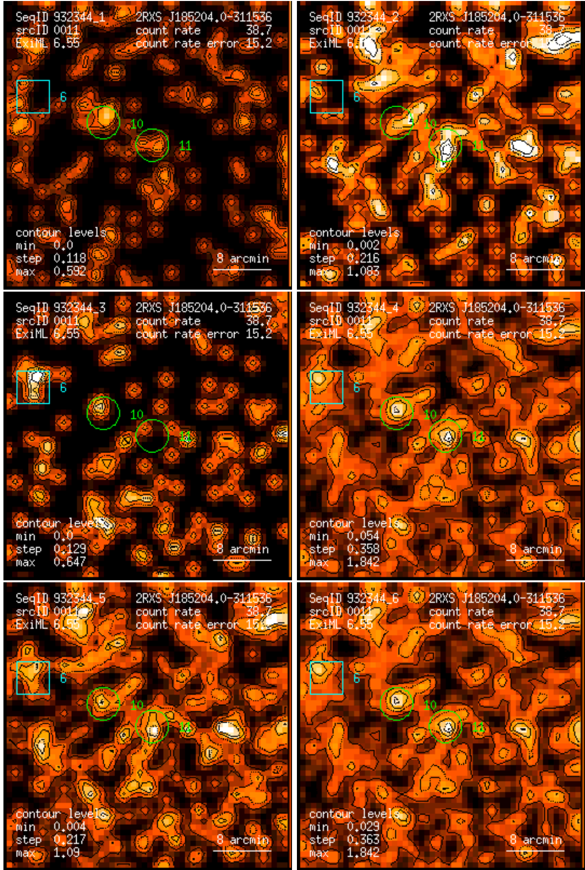
Figure 11: RASS 932344: detection 0011: band rate images, Gaussian filter: (1) PSPC channels 11 – 41, (2) 52 – 90, (3) 91 – 201, (4) 11 – 235, (5) 52 – 201, (6) 11 – 201. Broad band rates in counts/ks. Band rate contour levels in counts/ks/arcmin 2 .
