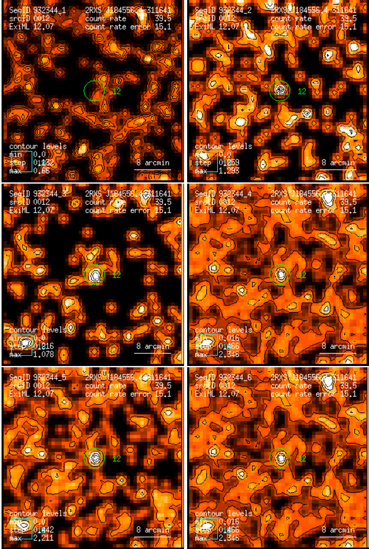
Figure 12: RASS 932344: detection 0012: band rate images, Gaussian filter: (1) PSPC channels 11 – 41, (2) 52 – 90, (3) 91 – 201, (4) 11 – 235, (5) 52 – 201, (6) 11 – 201. Broad band rates in counts/ks. Band rate contour levels in counts/ks/arcmin 2 .
