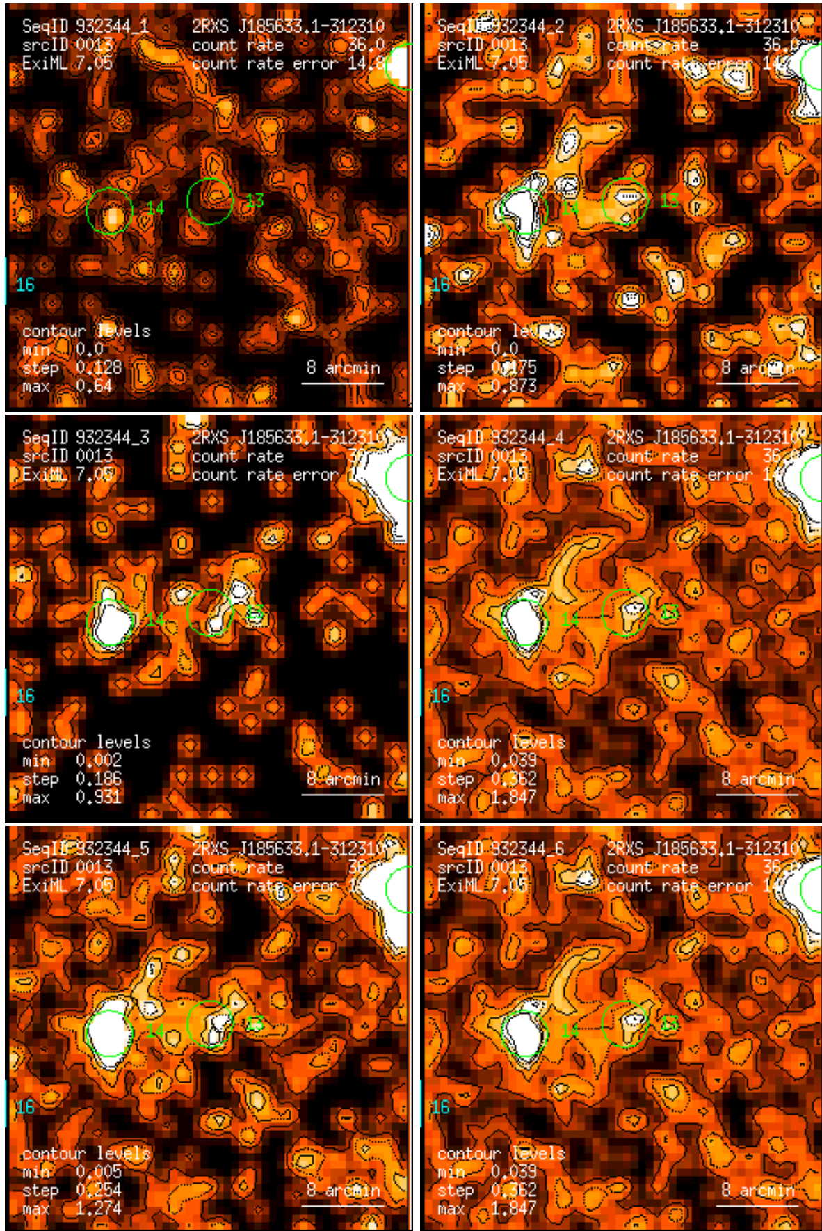
Figure 13: RASS 932344: detection 0013: band rate images, Gaussian filter: (1) PSPC channels 11 – 41, (2) 52 – 90, (3) 91 – 201, (4) 11 – 235, (5) 52 – 201, (6) 11 – 201. Broad band rates in counts/ks. Band rate contour levels in counts/ks/arcmin 2 .
