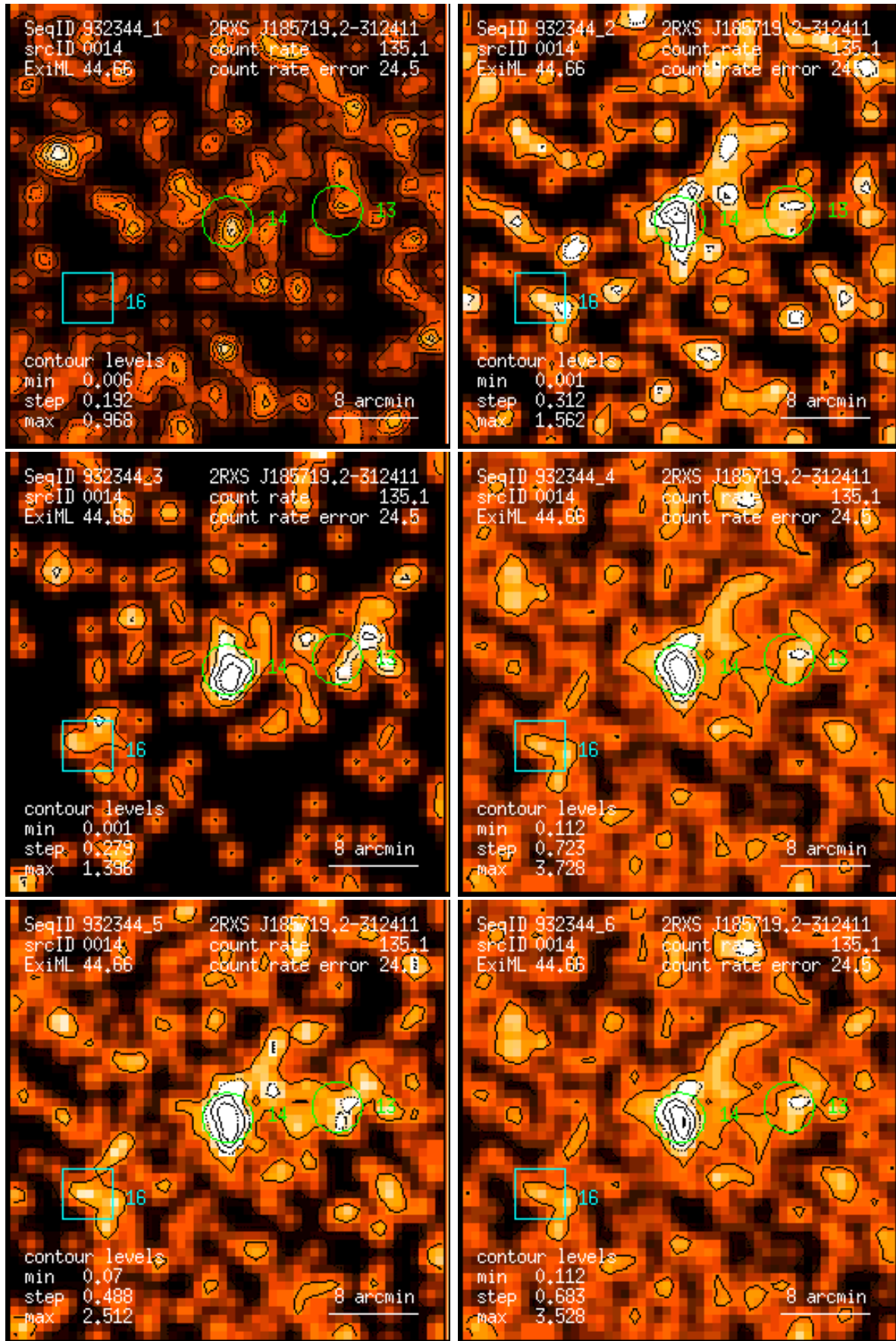
Figure 14: RASS 932344: detection 0014: band rate images, Gaussian filter: (1) PSPC channels 11 – 41, (2) 52 – 90, (3) 91 – 201, (4) 11 – 235, (5) 52 – 201, (6) 11 – 201. Broad band rates in counts/ks. Band rate contour levels in counts/ks/arcmin 2 .
