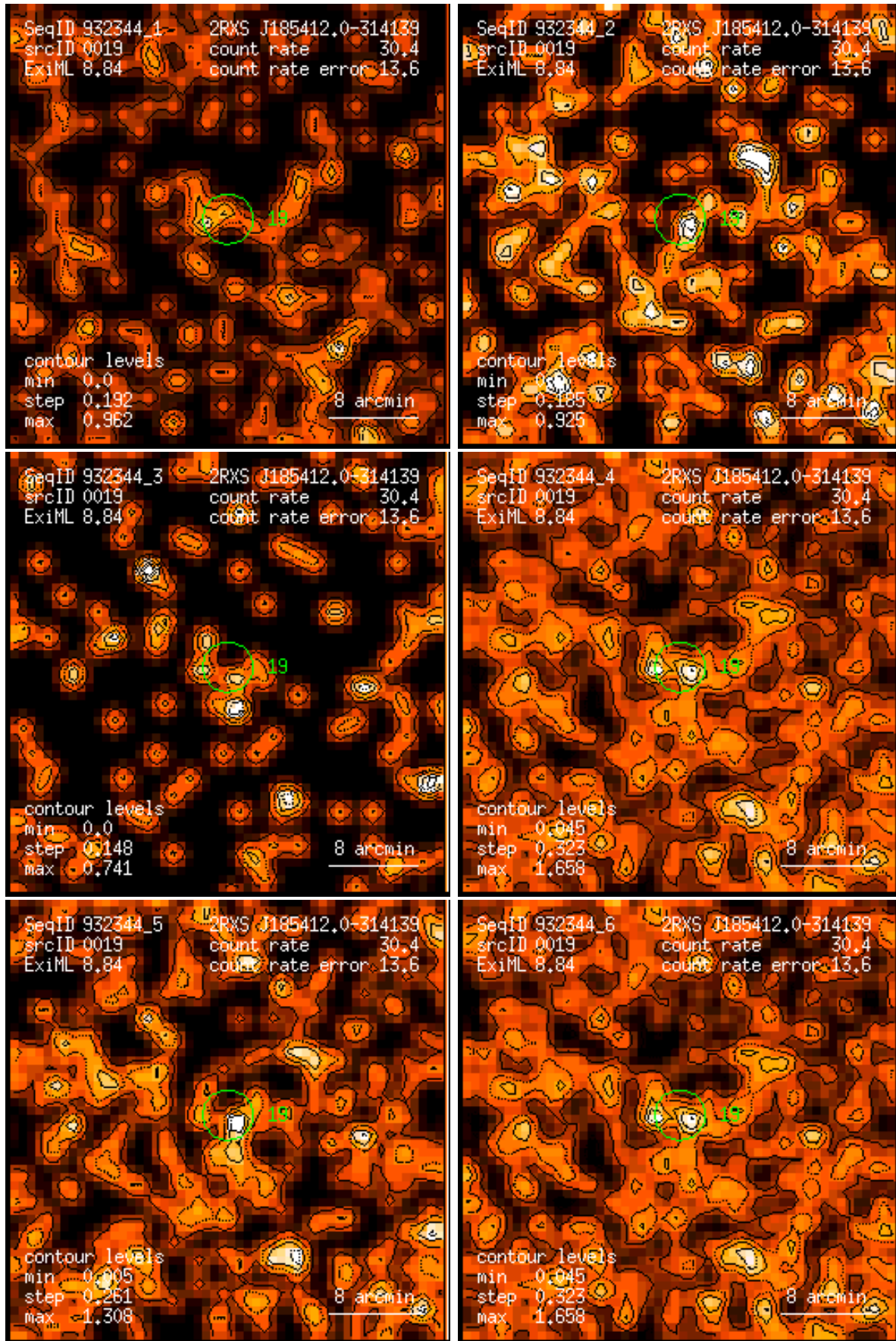
Figure 19: RASS 932344: detection 0019: band rate images, Gaussian filter: (1) PSPC channels 11 – 41, (2) 52 – 90, (3) 91 – 201, (4) 11 – 235, (5) 52 – 201, (6) 11 – 201. Broad band rates in counts/ks. Band rate contour levels in counts/ks/arcmin 2 .
