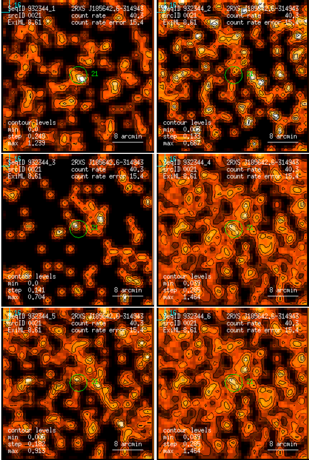
Figure 21: RASS 932344: detection 0021: band rate images, Gaussian filter: (1) PSPC channels 11 – 41, (2) 52 – 90, (3) 91 – 201, (4) 11 – 235, (5) 52 – 201, (6) 11 – 201. Broad band rates in counts/ks. Band rate contour levels in counts/ks/arcmin 2 .
