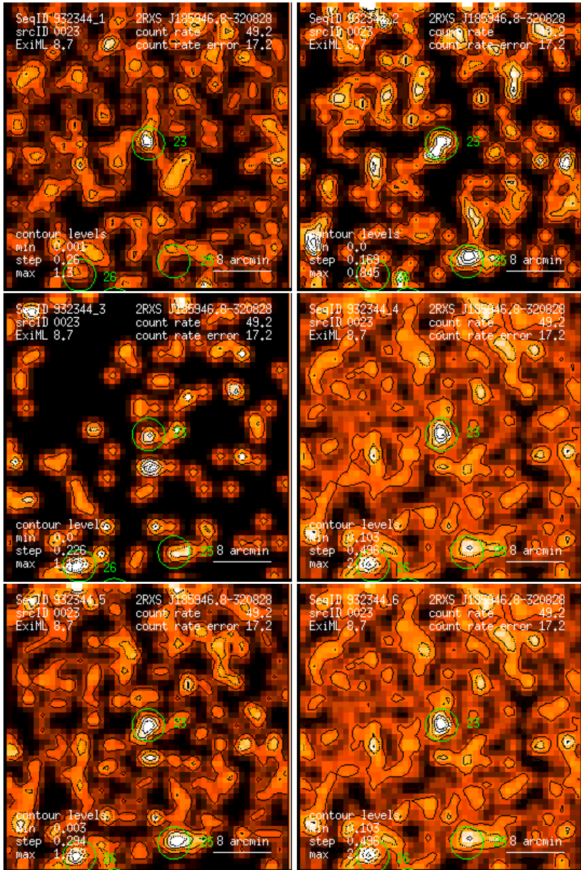
Figure 23: RASS 932344: detection 0023: band rate images, Gaussian filter: (1) PSPC channels 11 – 41, (2) 52 – 90, (3) 91 – 201, (4) 11 – 235, (5) 52 – 201, (6) 11 – 201. Broad band rates in counts/ks. Band rate contour levels in counts/ks/arcmin 2 .
