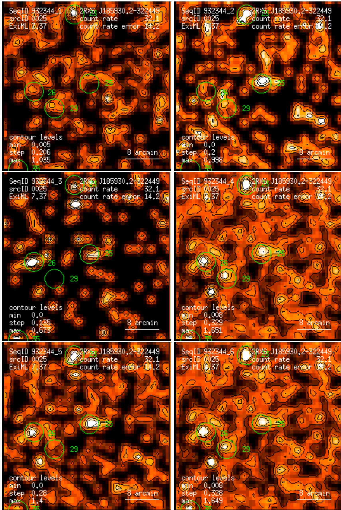
Figure 25: RASS 932344: detection 0025: band rate images, Gaussian filter: (1) PSPC channels 11 – 41, (2) 52 – 90, (3) 91 – 201, (4) 11 – 235, (5) 52 – 201, (6) 11 – 201. Broad band rates in counts/ks. Band rate contour levels in counts/ks/arcmin 2 .
