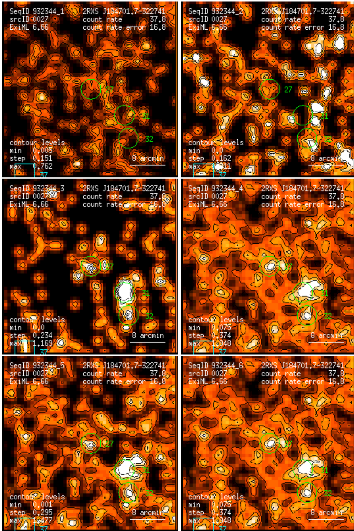
Figure 27: RASS 932344: detection 0027: band rate images, Gaussian filter: (1) PSPC channels 11 – 41, (2) 52 – 90, (3) 91 – 201, (4) 11 – 235, (5) 52 – 201, (6) 11 – 201. Broad band rates in counts/ks. Band rate contour levels in counts/ks/arcmin 2 .
