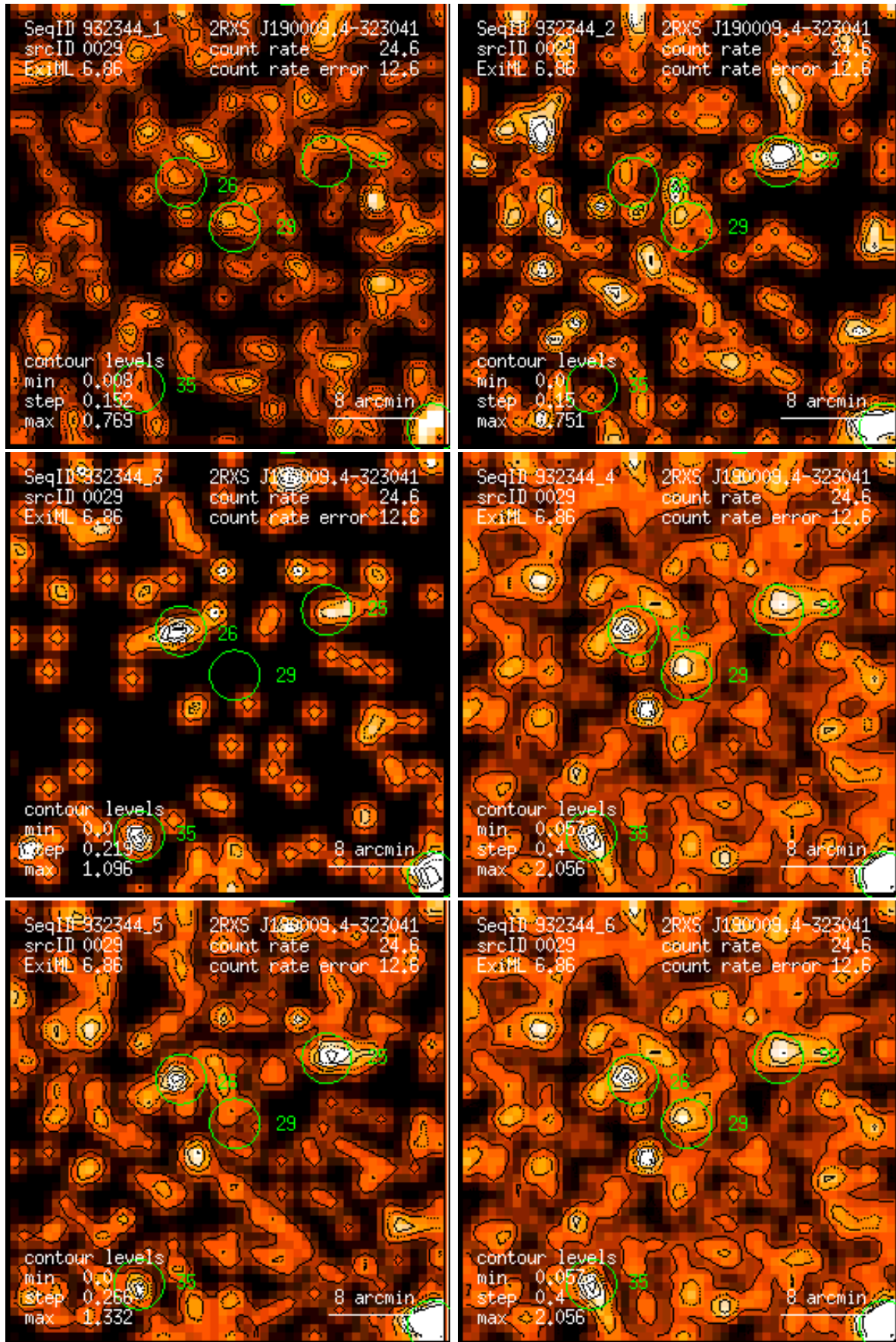
Figure 29: RASS 932344: detection 0029: band rate images, Gaussian filter: (1) PSPC channels 11 – 41, (2) 52 – 90, (3) 91 – 201, (4) 11 – 235, (5) 52 – 201, (6) 11 – 201. Broad band rates in counts/ks. Band rate contour levels in counts/ks/arcmin 2 .
