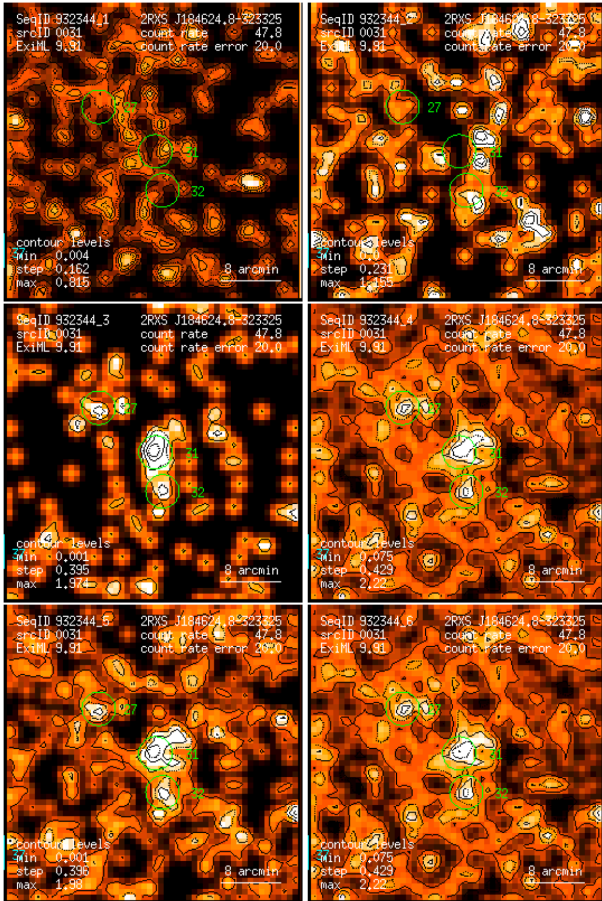
Figure 31: RASS 932344: detection 0031: band rate images, Gaussian filter: (1) PSPC channels 11 – 41, (2) 52 – 90, (3) 91 – 201, (4) 11 – 235, (5) 52 – 201, (6) 11 – 201. Broad band rates in counts/ks. Band rate contour levels in counts/ks/arcmin 2 .
