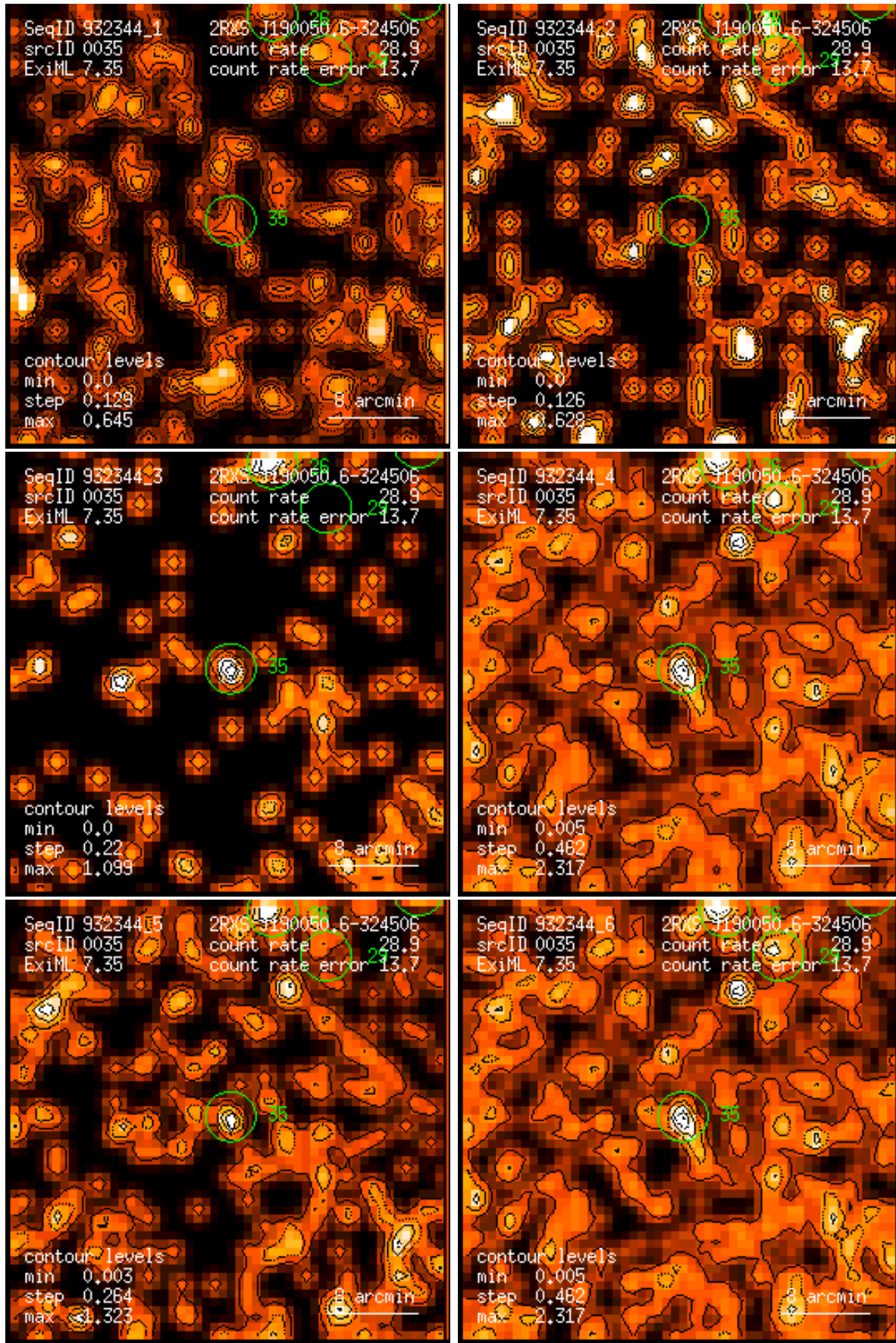
Figure 35: RASS 932344: detection 0035: band rate images, Gaussian filter: (1) PSPC channels 11 – 41, (2) 52 – 90, (3) 91 – 201, (4) 11 – 235, (5) 52 – 201, (6) 11 – 201. Broad band rates in counts/ks. Band rate contour levels in counts/ks/arcmin 2 .
