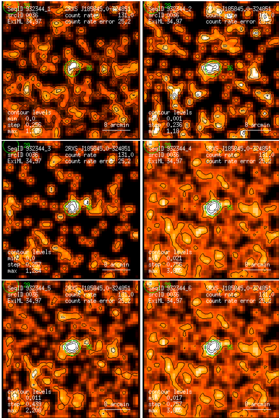
Figure 36: RASS 932344: detection 0036: band rate images, Gaussian filter: (1) PSPC channels 11 – 41, (2) 52 – 90, (3) 91 – 201, (4) 11 – 235, (5) 52 – 201, (6) 11 – 201. Broad band rates in counts/ks. Band rate contour levels in counts/ks/arcmin 2 .
