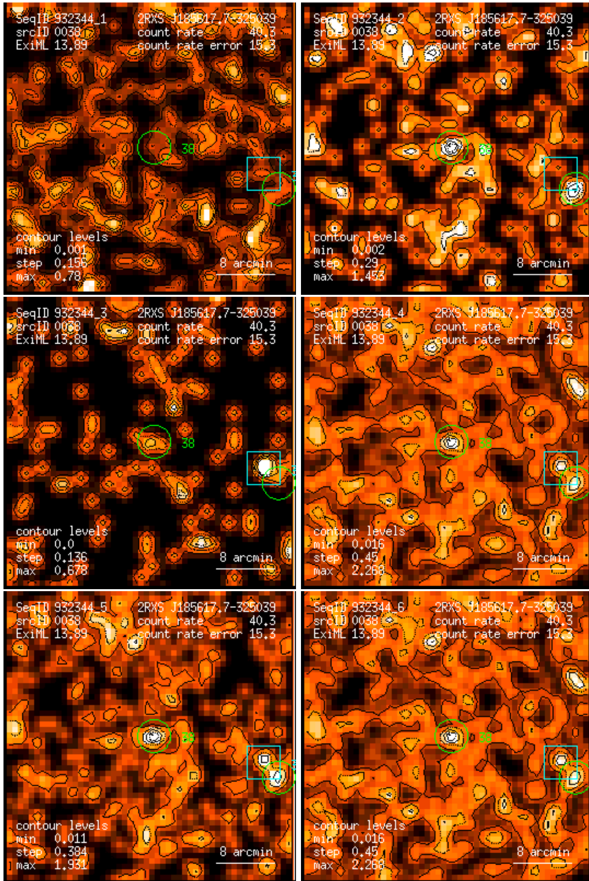
Figure 38: RASS 932344: detection 0038: band rate images, Gaussian filter: (1) PSPC channels 11 – 41, (2) 52 – 90, (3) 91 – 201, (4) 11 – 235, (5) 52 – 201, (6) 11 – 201. Broad band rates in counts/ks. Band rate contour levels in counts/ks/arcmin 2 .
