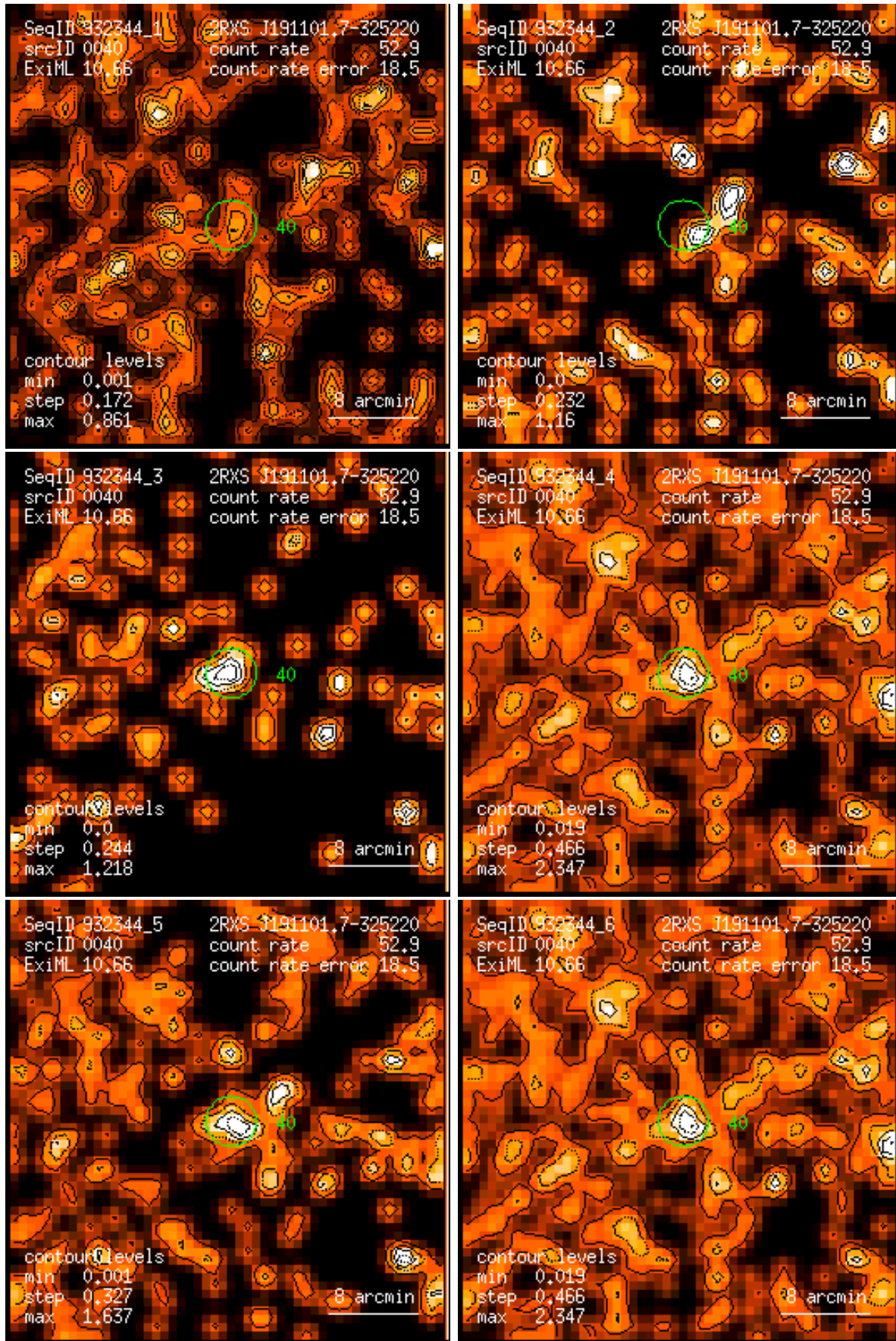
Figure 40: RASS 932344: detection 0040: band rate images, Gaussian filter: (1) PSPC channels 11 – 41, (2) 52 – 90, (3) 91 – 201, (4) 11 – 235, (5) 52 – 201, (6) 11 – 201. Broad band rates in counts/ks. Band rate contour levels in counts/ks/arcmin 2 .
