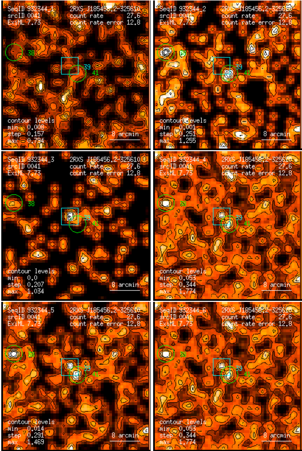
Figure 41: RASS 932344: detection 0041: band rate images, Gaussian filter: (1) PSPC channels 11 – 41, (2) 52 – 90, (3) 91 – 201, (4) 11 – 235, (5) 52 – 201, (6) 11 – 201. Broad band rates in counts/ks. Band rate contour levels in counts/ks/arcmin 2 .
