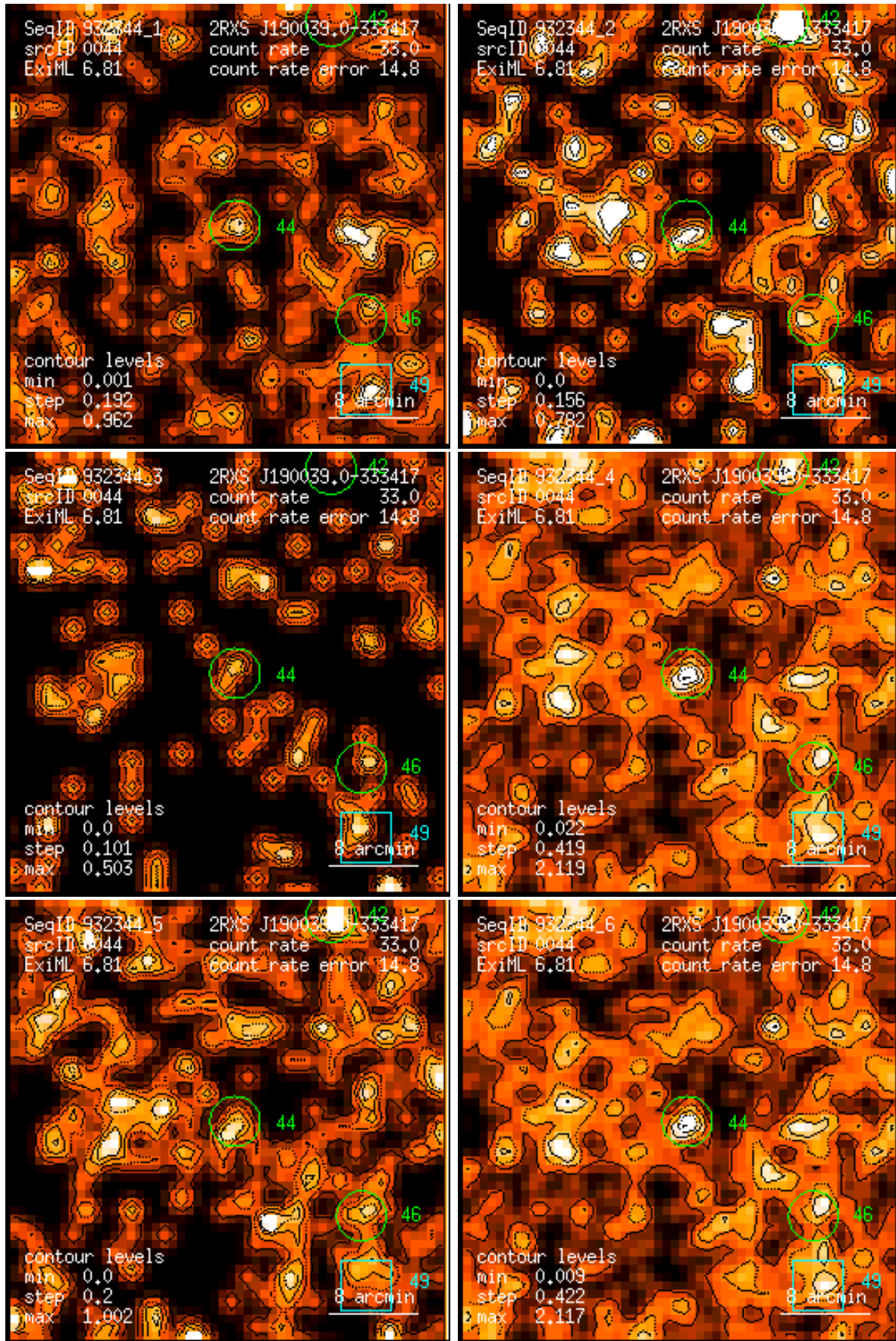
Figure 44: RASS 932344: detection 0044: band rate images, Gaussian filter: (1) PSPC channels 11 – 41, (2) 52 – 90, (3) 91 – 201, (4) 11 – 235, (5) 52 – 201, (6) 11 – 201. Broad band rates in counts/ks. Band rate contour levels in counts/ks/arcmin 2 .
