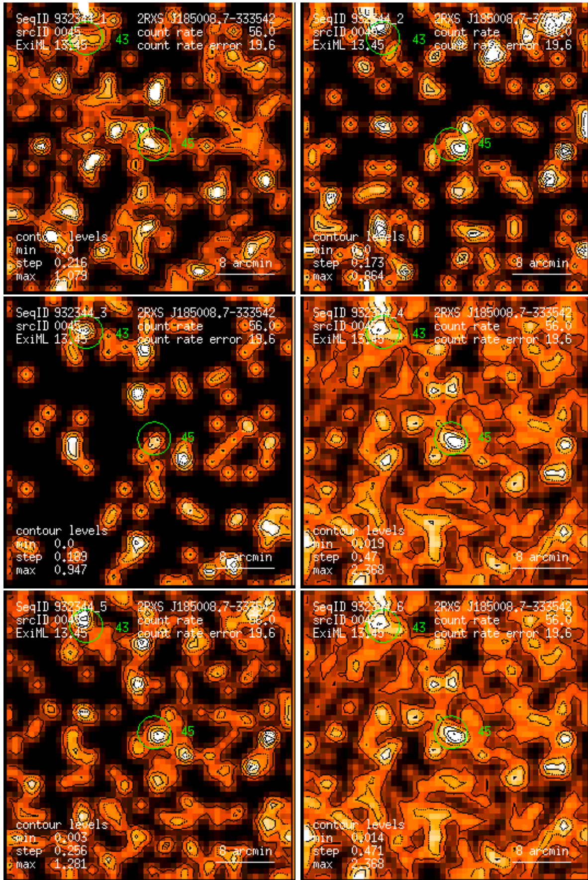
Figure 45: RASS 932344: detection 0045: band rate images, Gaussian filter: (1) PSPC channels 11 – 41, (2) 52 – 90, (3) 91 – 201, (4) 11 – 235, (5) 52 – 201, (6) 11 – 201. Broad band rates in counts/ks. Band rate contour levels in counts/ks/arcmin 2 .
