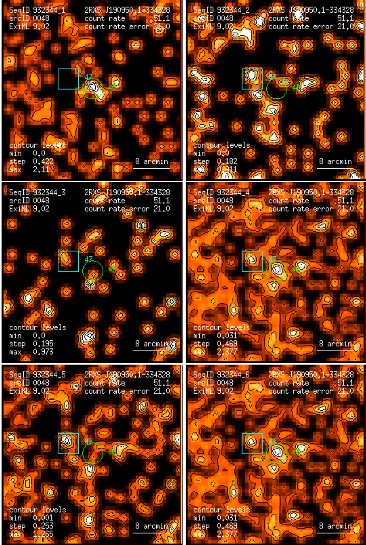
Figure 48: RASS 932344: detection 0048: band rate images, Gaussian filter: (1) PSPC channels 11 – 41, (2) 52 – 90, (3) 91 – 201, (4) 11 – 235, (5) 52 – 201, (6) 11 – 201. Broad band rates in counts/ks. Band rate contour levels in counts/ks/arcmin 2 .
