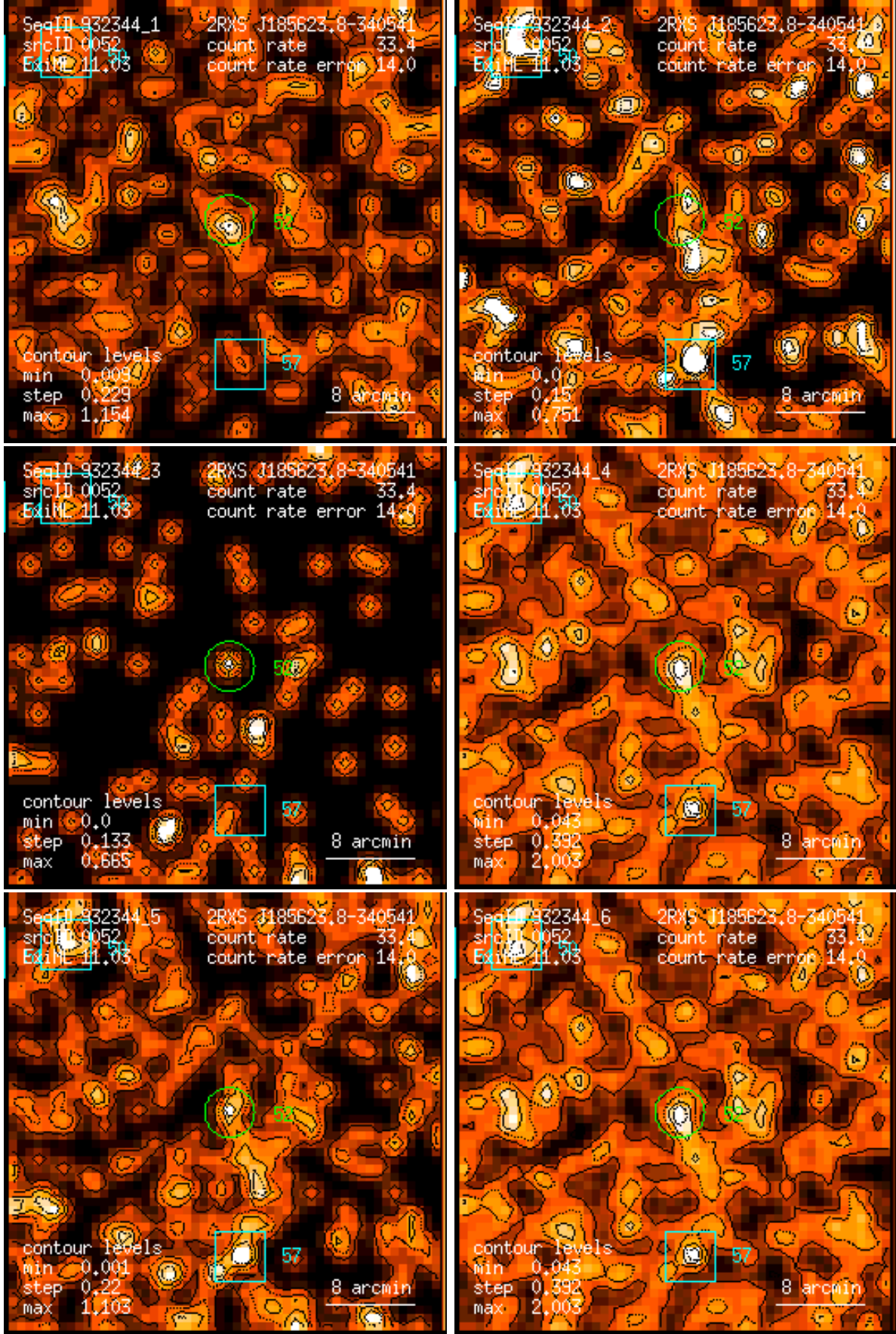
Figure 52: RASS 932344: detection 0052: band rate images, Gaussian filter: (1) PSPC channels 11 – 41, (2) 52 – 90, (3) 91 – 201, (4) 11 – 235, (5) 52 – 201, (6) 11 – 201. Broad band rates in counts/ks. Band rate contour levels in counts/ks/arcmin 2 .
