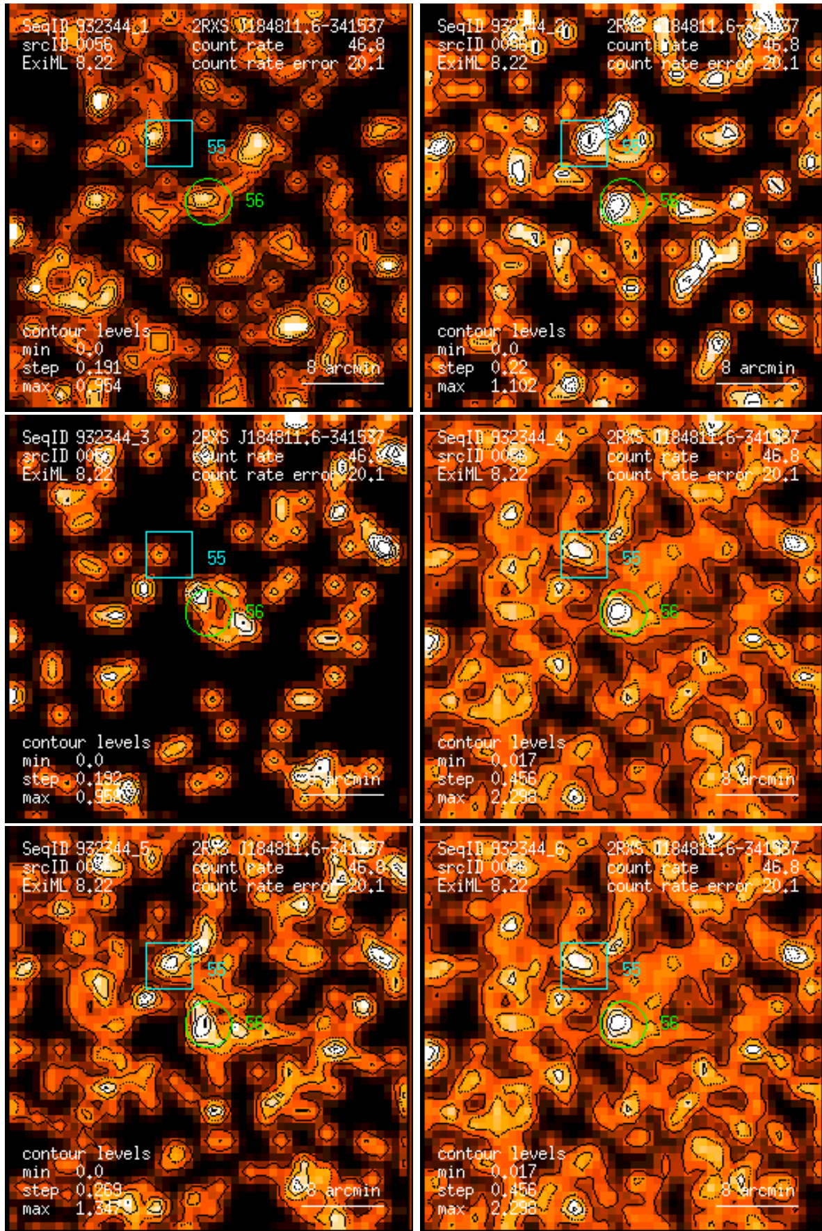
Figure 56: RASS 932344: detection 0056: band rate images, Gaussian filter: (1) PSPC channels 11 – 41, (2) 52 – 90, (3) 91 – 201, (4) 11 – 235, (5) 52 – 201, (6) 11 – 201. Broad band rates in counts/ks. Band rate contour levels in counts/ks/arcmin 2 .
