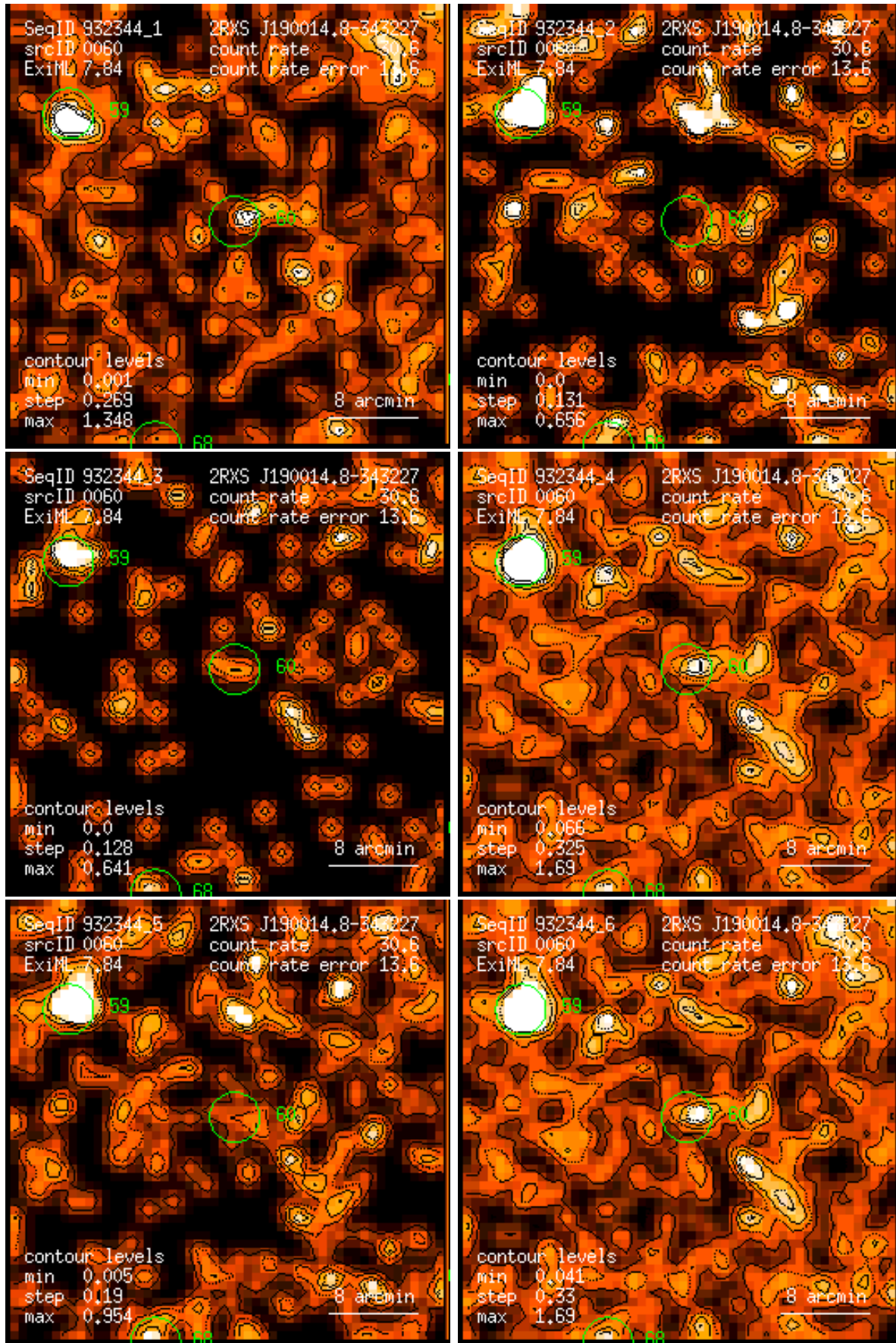
Figure 60: RASS 932344: detection 0060: band rate images, Gaussian filter: (1) PSPC channels 11 – 41, (2) 52 – 90, (3) 91 – 201, (4) 11 – 235, (5) 52 – 201, (6) 11 – 201. Broad band rates in counts/ks. Band rate contour levels in counts/ks/arcmin 2 .
