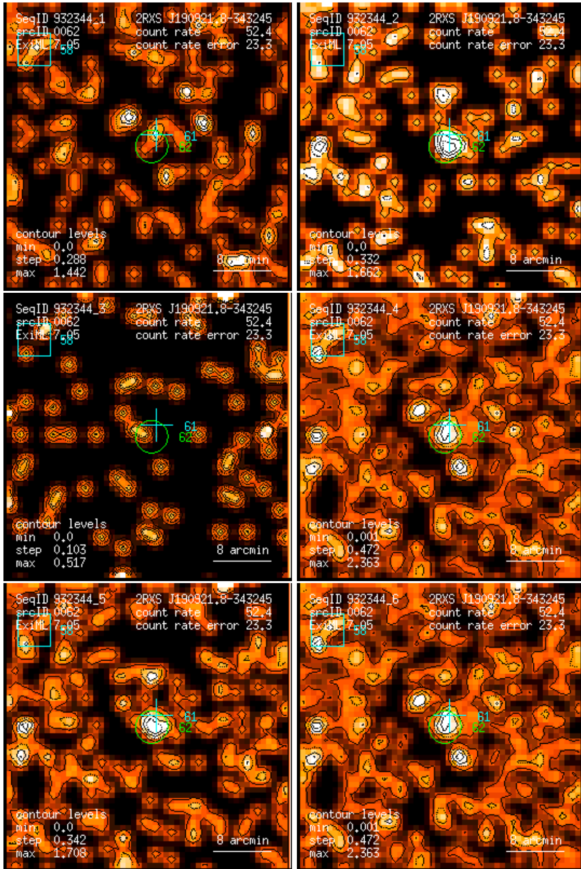
Figure 62: RASS 932344: detection 0062: band rate images, Gaussian filter: (1) PSPC channels 11 – 41, (2) 52 – 90, (3) 91 – 201, (4) 11 – 235, (5) 52 – 201, (6) 11 – 201. Broad band rates in counts/ks. Band rate contour levels in counts/ks/arcmin 2 .
