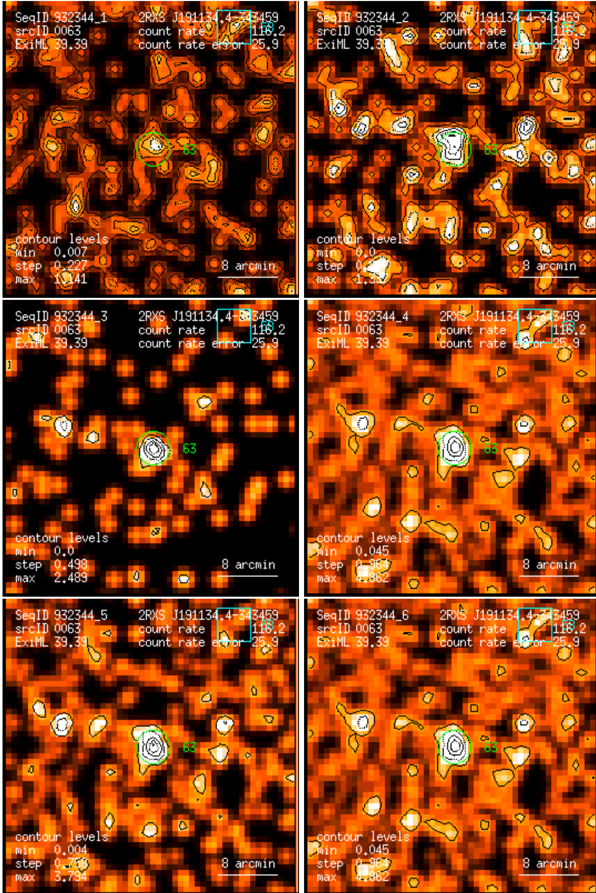
Figure 63: RASS 932344: detection 0063: band rate images, Gaussian filter: (1) PSPC channels 11 – 41, (2) 52 – 90, (3) 91 – 201, (4) 11 – 235, (5) 52 – 201, (6) 11 – 201. Broad band rates in counts/ks. Band rate contour levels in counts/ks/arcmin 2 .
