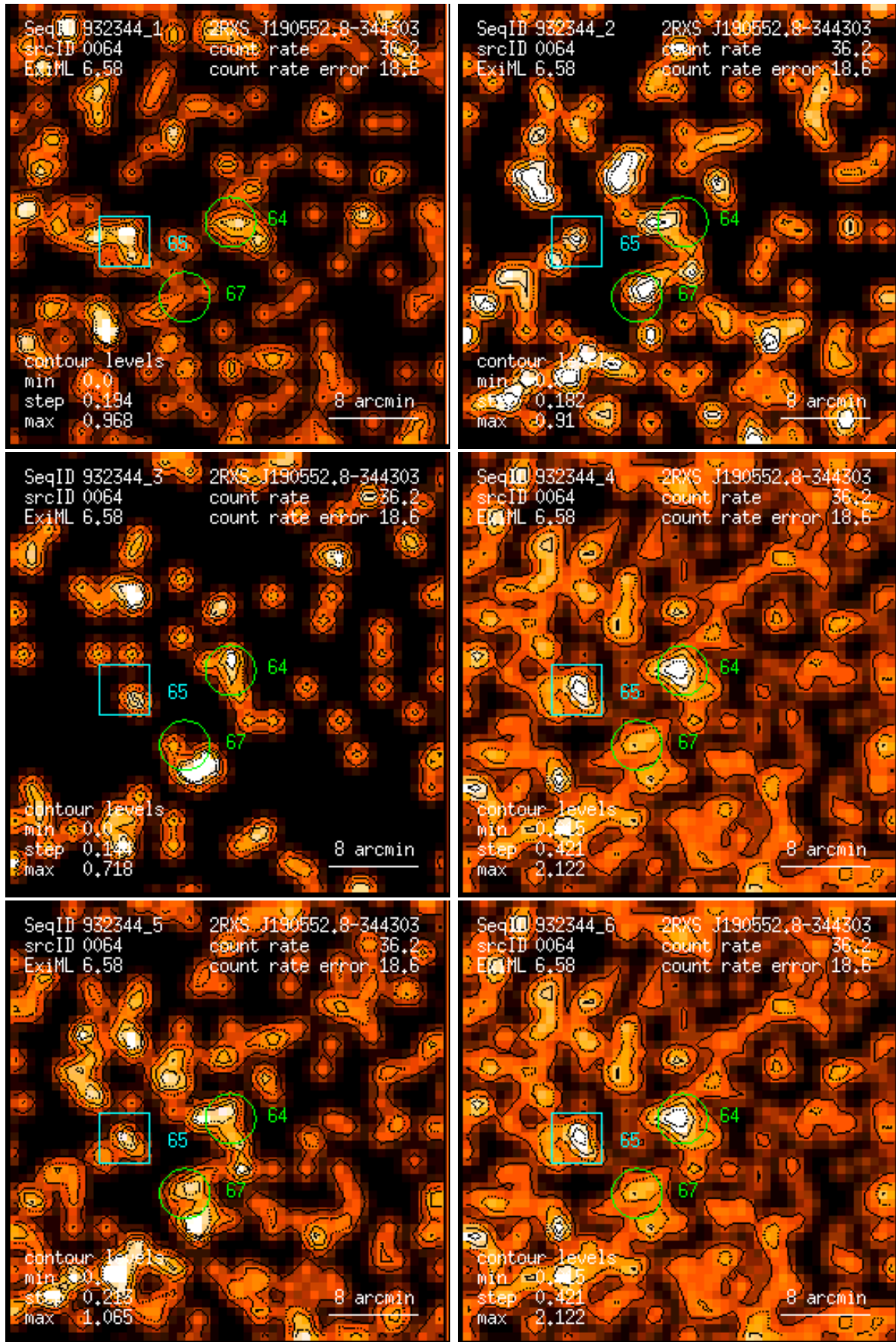
Figure 64: RASS 932344: detection 0064: band rate images, Gaussian filter: (1) PSPC channels 11 – 41, (2) 52 – 90, (3) 91 – 201, (4) 11 – 235, (5) 52 – 201, (6) 11 – 201. Broad band rates in counts/ks. Band rate contour levels in counts/ks/arcmin 2 .
