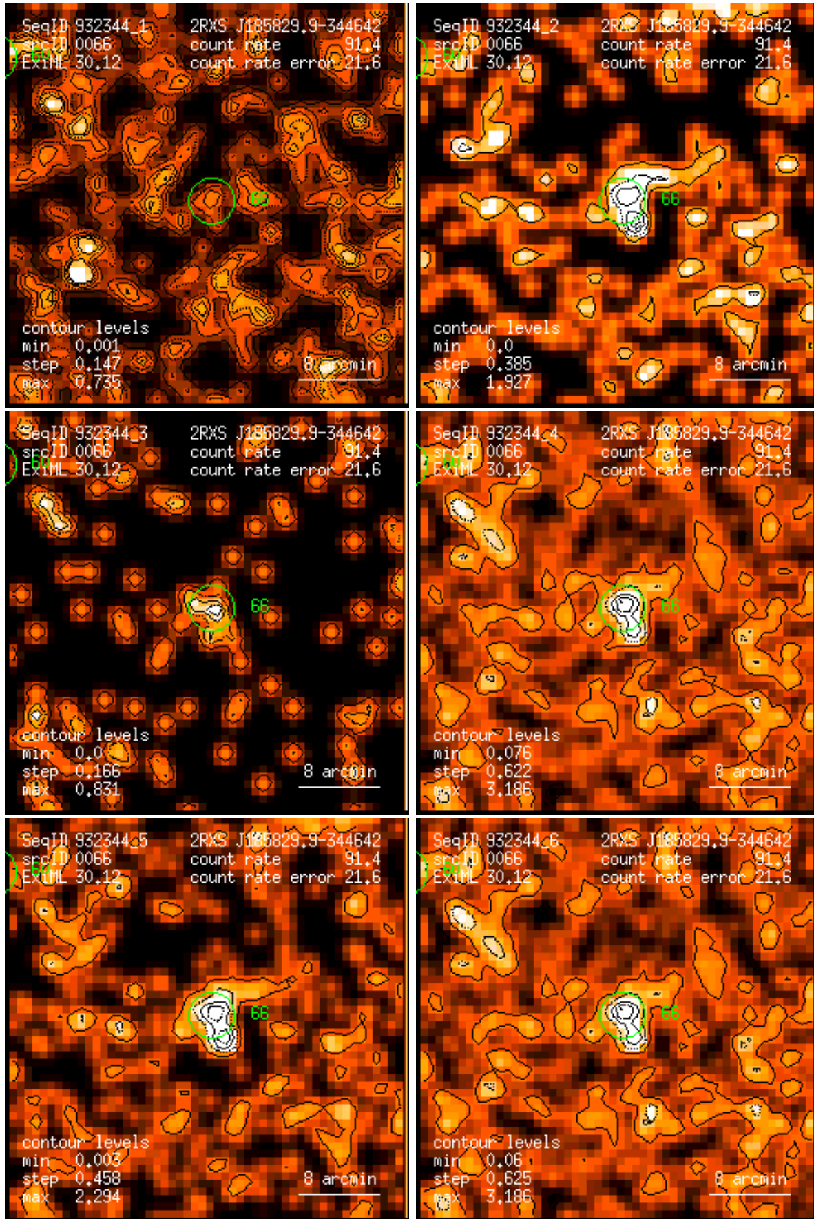
Figure 66: RASS 932344: detection 0066: band rate images, Gaussian filter: (1) PSPC channels 11 – 41, (2) 52 – 90, (3) 91 – 201, (4) 11 – 235, (5) 52 – 201, (6) 11 – 201. Broad band rates in counts/ks. Band rate contour levels in counts/ks/arcmin 2 .
