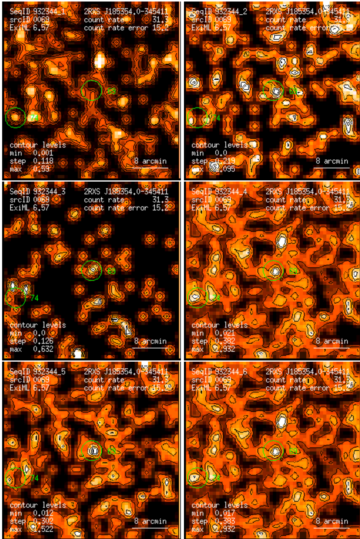
Figure 69: RASS 932344: detection 0069: band rate images, Gaussian filter: (1) PSPC channels 11 – 41, (2) 52 – 90, (3) 91 – 201, (4) 11 – 235, (5) 52 – 201, (6) 11 – 201. Broad band rates in counts/ks. Band rate contour levels in counts/ks/arcmin 2 .
