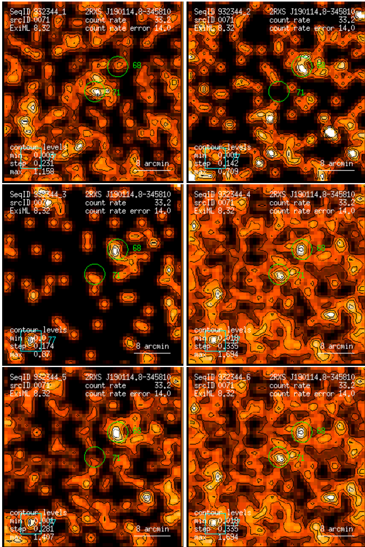
Figure 71: RASS 932344: detection 0071: band rate images, Gaussian filter: (1) PSPC channels 11 – 41, (2) 52 – 90, (3) 91 – 201, (4) 11 – 235, (5) 52 – 201, (6) 11 – 201. Broad band rates in counts/ks. Band rate contour levels in counts/ks/arcmin 2 .
