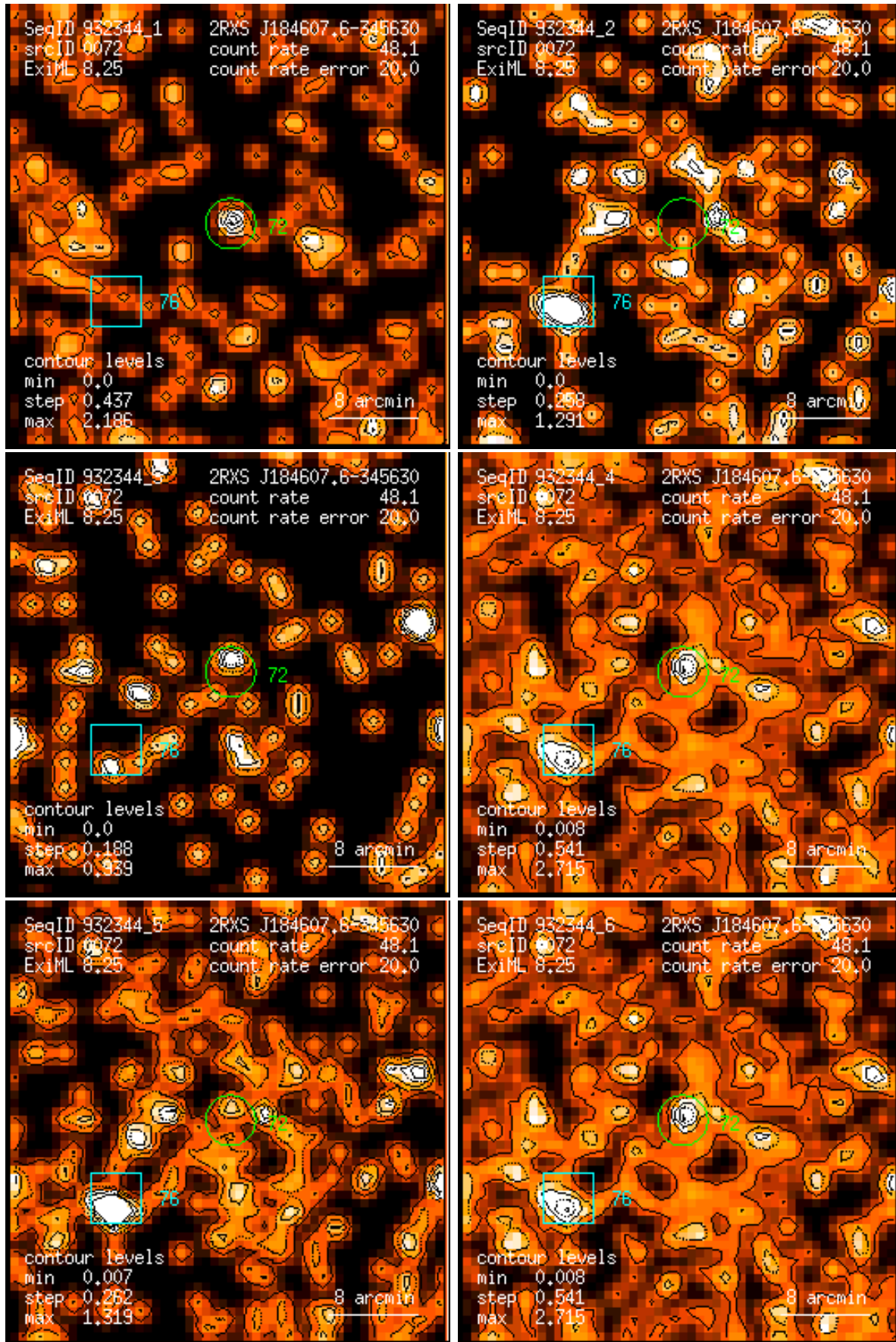
Figure 72: RASS 932344: detection 0072: band rate images, Gaussian filter: (1) PSPC channels 11 – 41, (2) 52 – 90, (3) 91 – 201, (4) 11 – 235, (5) 52 – 201, (6) 11 – 201. Broad band rates in counts/ks. Band rate contour levels in counts/ks/arcmin 2 .
