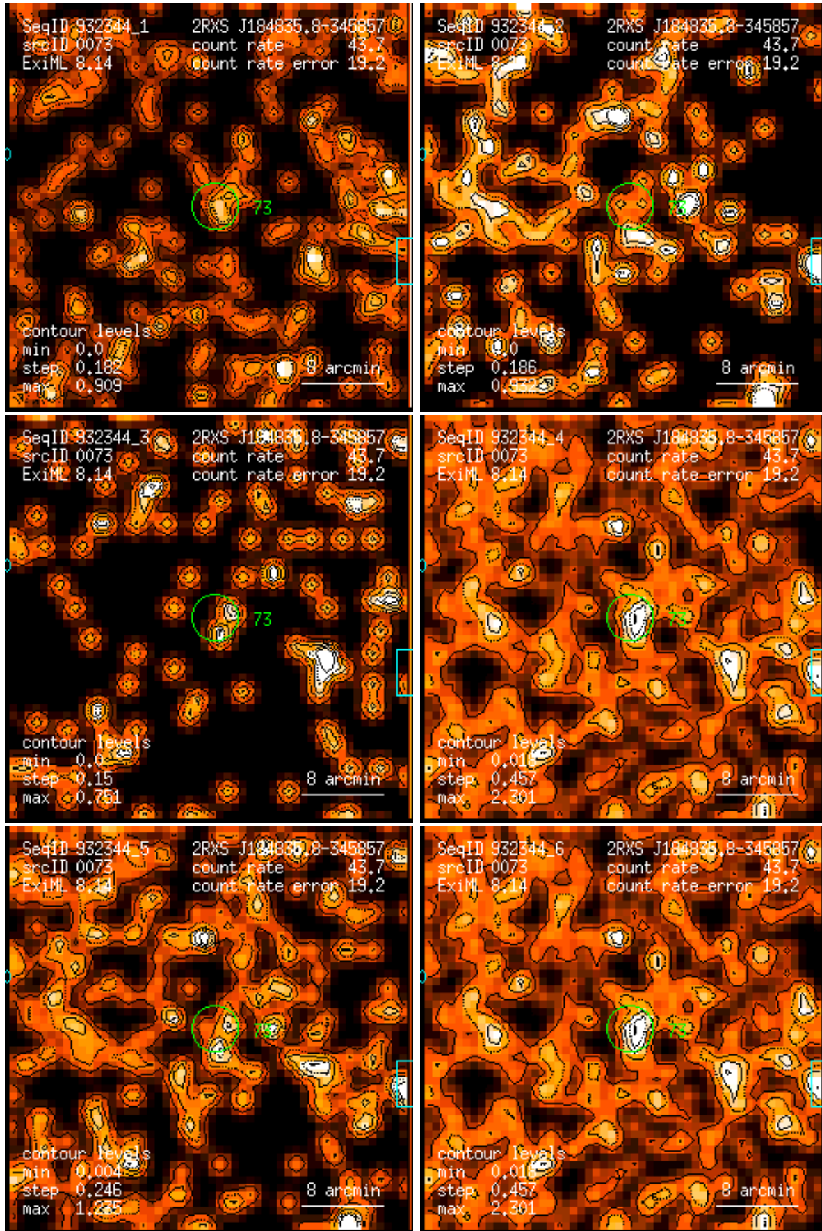
Figure 73: RASS 932344: detection 0073: band rate images, Gaussian filter: (1) PSPC channels 11 – 41, (2) 52 – 90, (3) 91 – 201, (4) 11 – 235, (5) 52 – 201, (6) 11 – 201. Broad band rates in counts/ks. Band rate contour levels in counts/ks/arcmin 2 .
