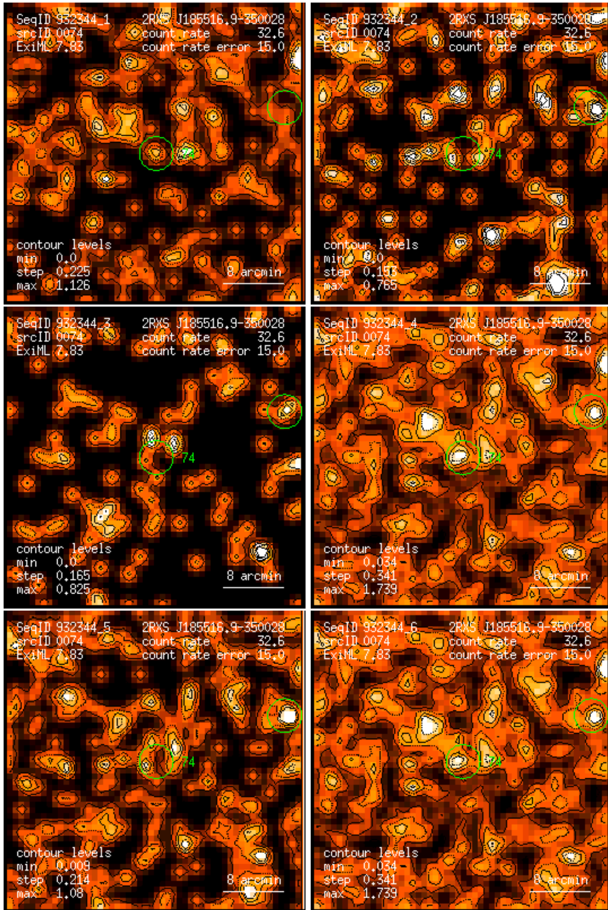
Figure 74: RASS 932344: detection 0074: band rate images, Gaussian filter: (1) PSPC channels 11 – 41, (2) 52 – 90, (3) 91 – 201, (4) 11 – 235, (5) 52 – 201, (6) 11 – 201. Broad band rates in counts/ks. Band rate contour levels in counts/ks/arcmin 2 .
