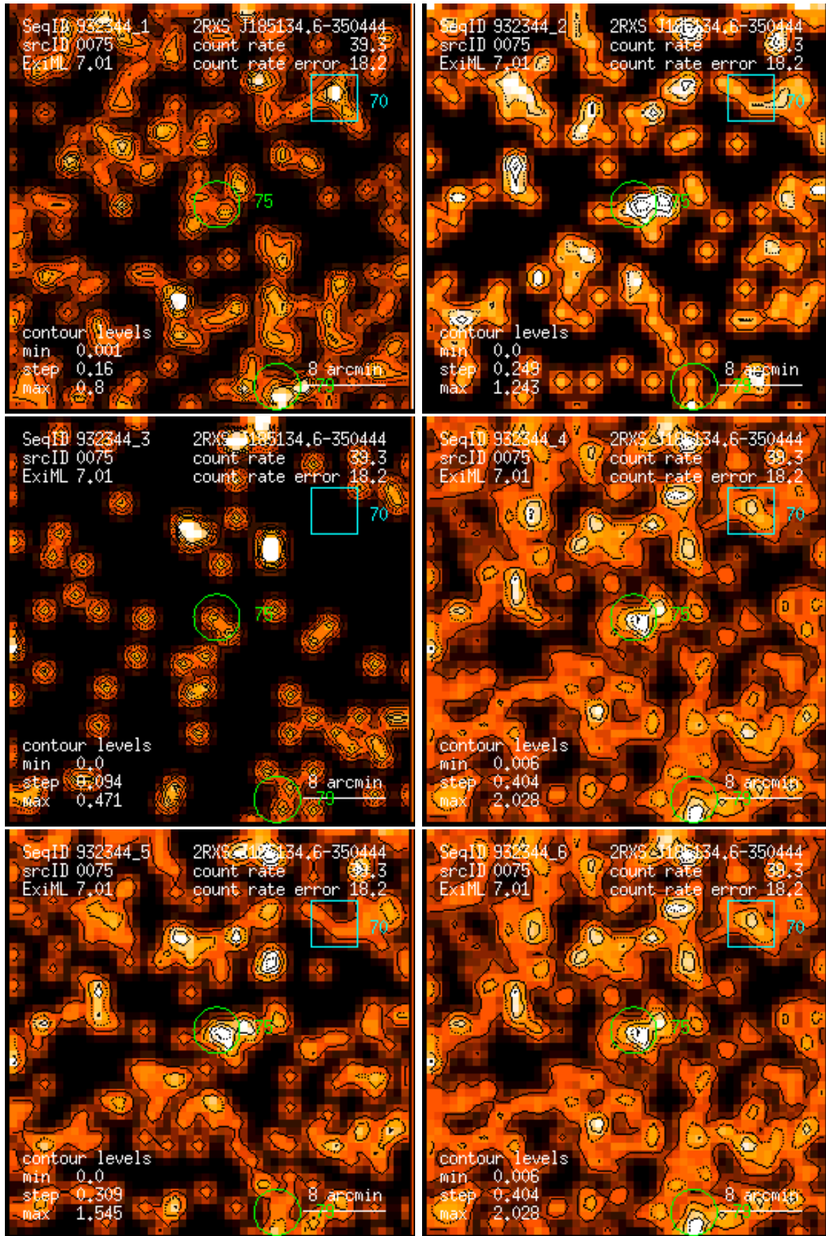
Figure 75: RASS 932344: detection 0075: band rate images, Gaussian filter: (1) PSPC channels 11 – 41, (2) 52 – 90, (3) 91 – 201, (4) 11 – 235, (5) 52 – 201, (6) 11 – 201. Broad band rates in counts/ks. Band rate contour levels in counts/ks/arcmin 2 .
