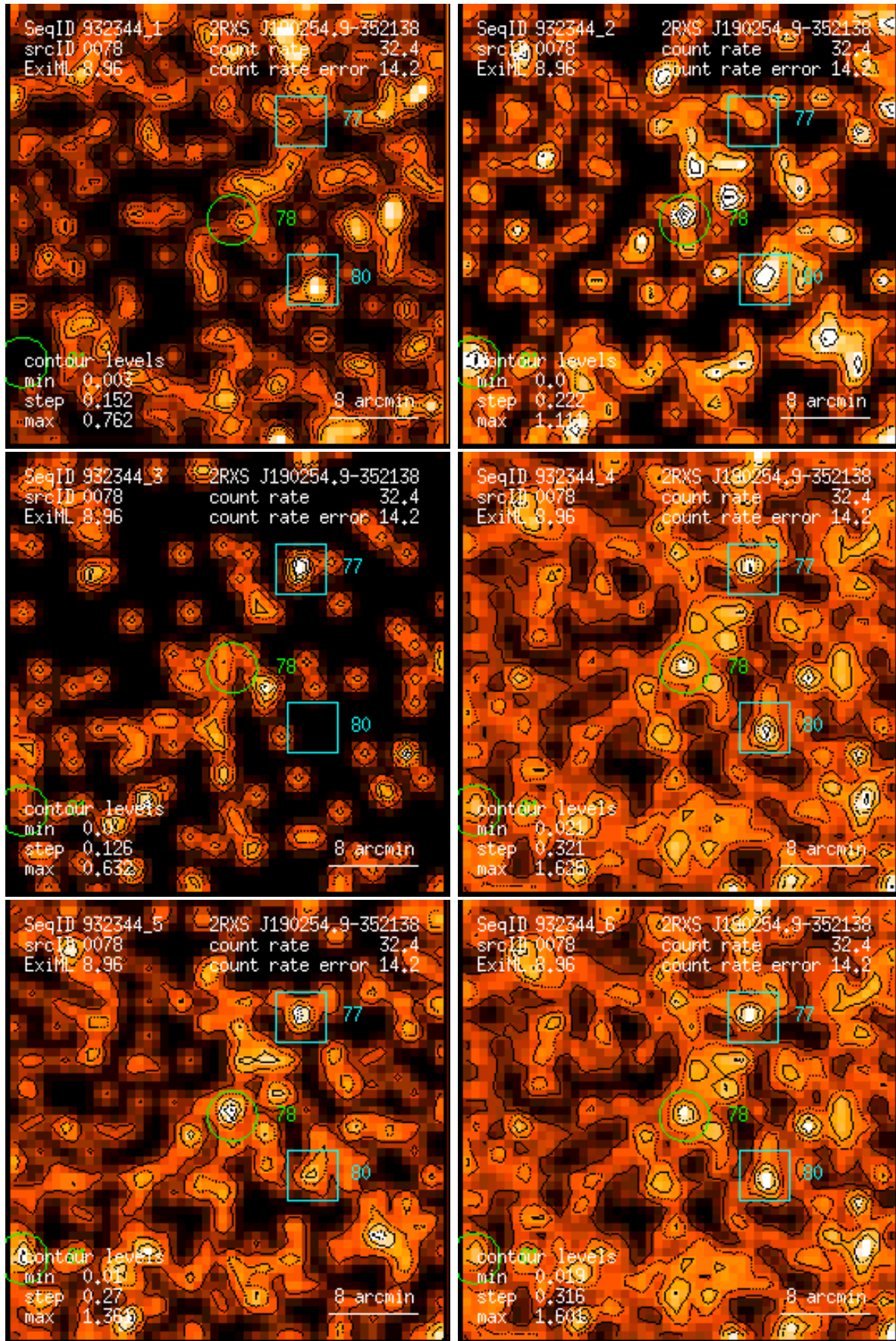
Figure 78: RASS 932344: detection 0078: band rate images, Gaussian filter: (1) PSPC channels 11 – 41, (2) 52 – 90, (3) 91 – 201, (4) 11 – 235, (5) 52 – 201, (6) 11 – 201. Broad band rates in counts/ks. Band rate contour levels in counts/ks/arcmin 2 .
