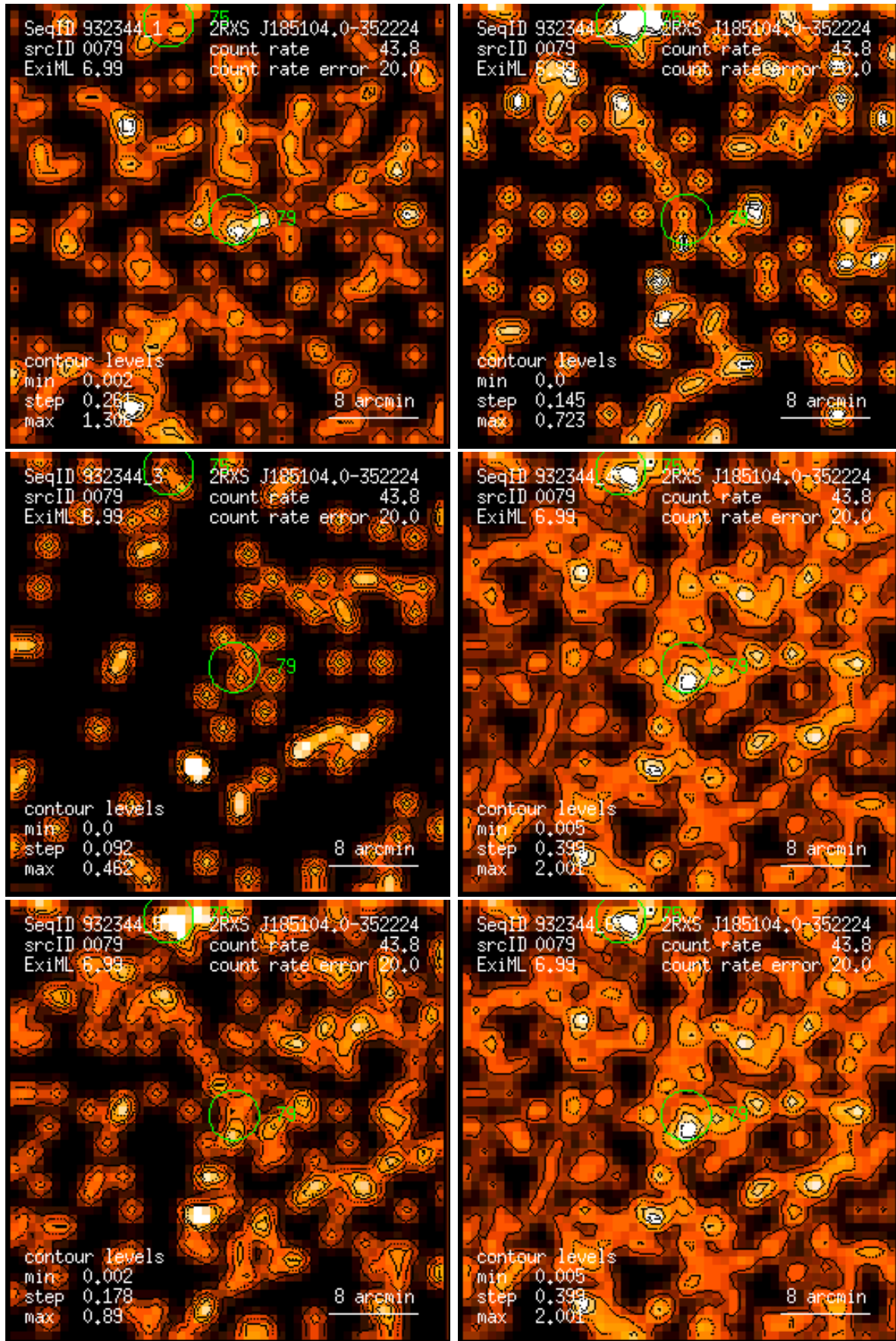
Figure 79: RASS 932344: detection 0079: band rate images, Gaussian filter: (1) PSPC channels 11 – 41, (2) 52 – 90, (3) 91 – 201, (4) 11 – 235, (5) 52 – 201, (6) 11 – 201. Broad band rates in counts/ks. Band rate contour levels in counts/ks/arcmin 2 .
