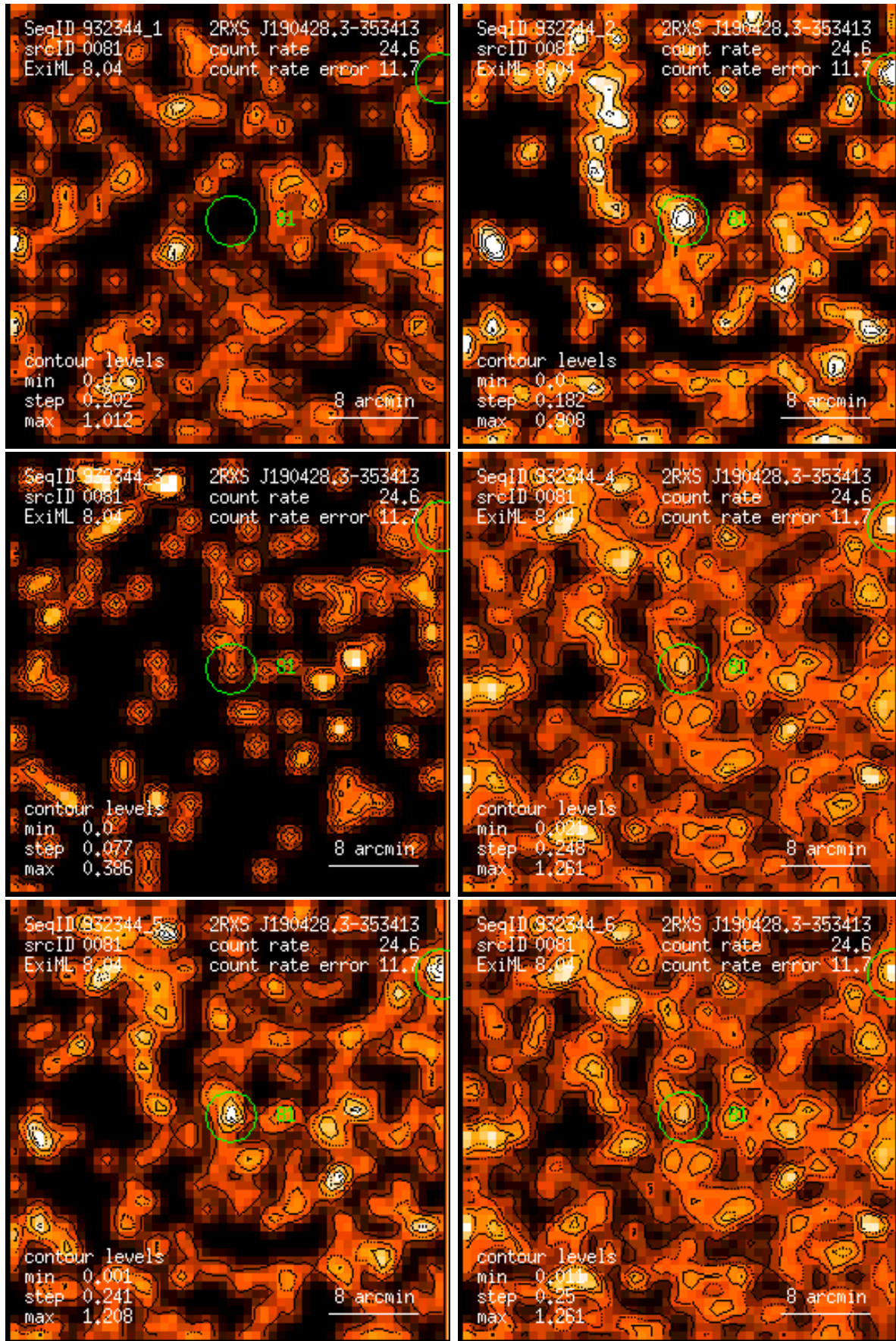
Figure 81: RASS 932344: detection 0081: band rate images, Gaussian filter: (1) PSPC channels 11 – 41, (2) 52 – 90, (3) 91 – 201, (4) 11 – 235, (5) 52 – 201, (6) 11 – 201. Broad band rates in counts/ks. Band rate contour levels in counts/ks/arcmin 2 .
