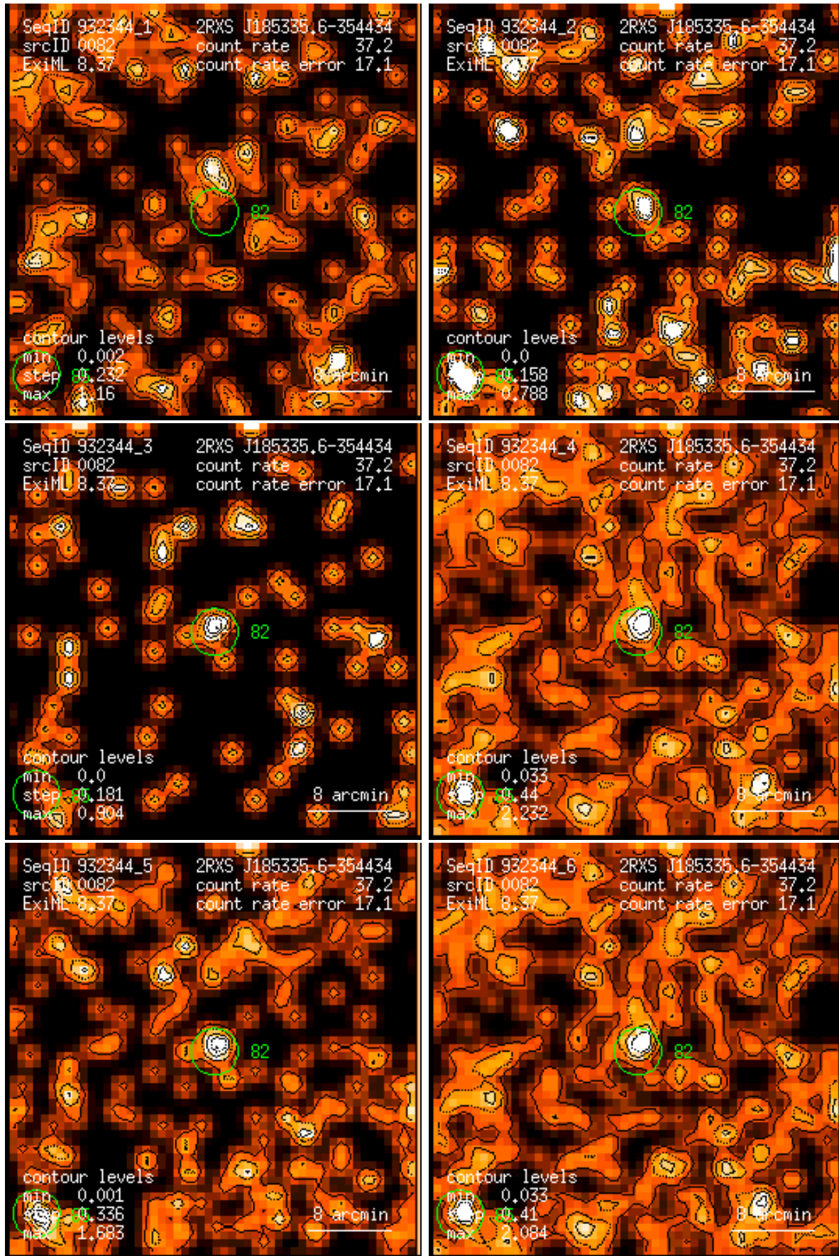
Figure 82: RASS 932344: detection 0082: band rate images, Gaussian filter: (1) PSPC channels 11 – 41, (2) 52 – 90, (3) 91 – 201, (4) 11 – 235, (5) 52 – 201, (6) 11 – 201. Broad band rates in counts/ks. Band rate contour levels in counts/ks/arcmin 2 .
