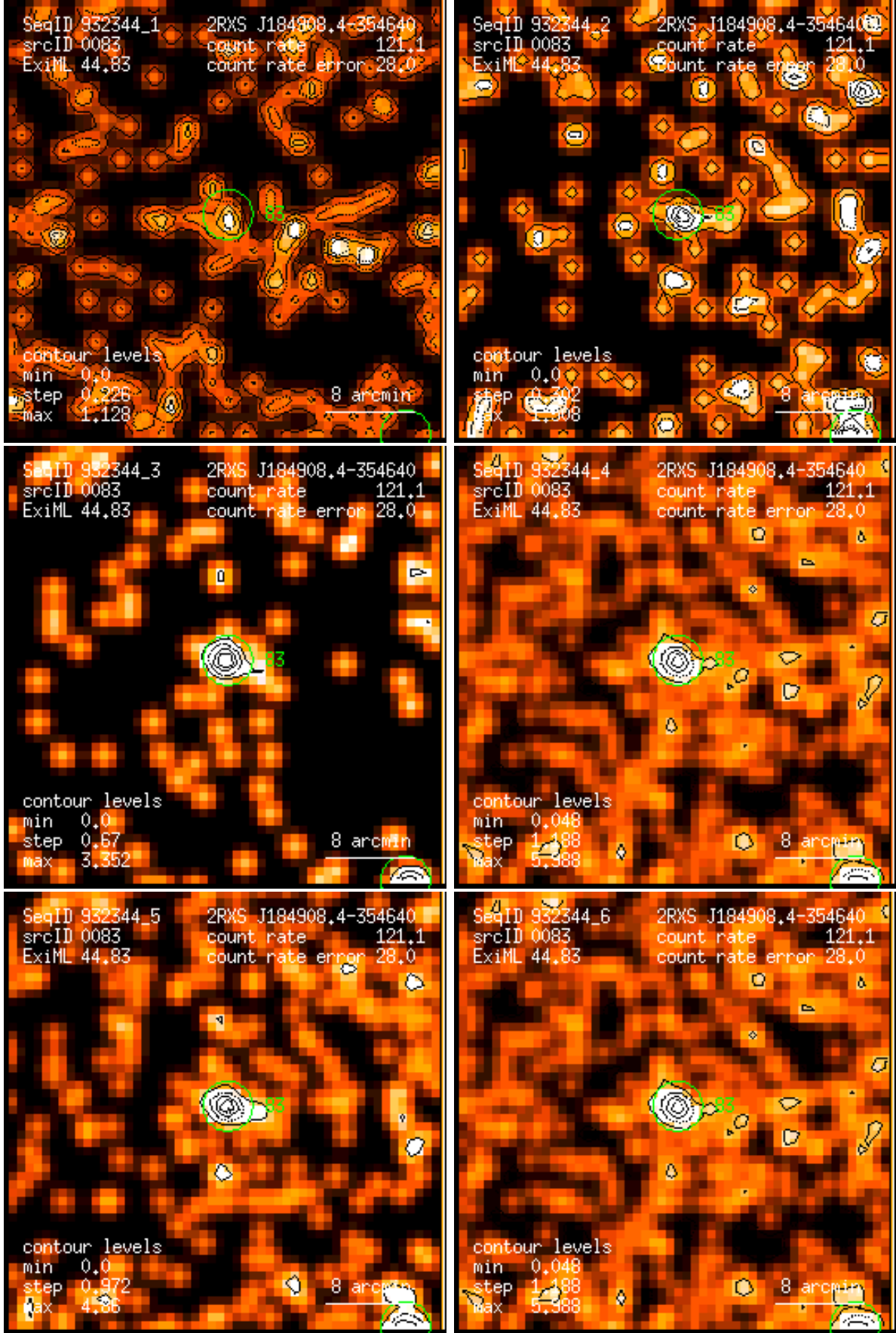
Figure 83: RASS 932344: detection 0083: band rate images, Gaussian filter: (1) PSPC channels 11 – 41, (2) 52 – 90, (3) 91 – 201, (4) 11 – 235, (5) 52 – 201, (6) 11 – 201. Broad band rates in counts/ks. Band rate contour levels in counts/ks/arcmin 2 .
