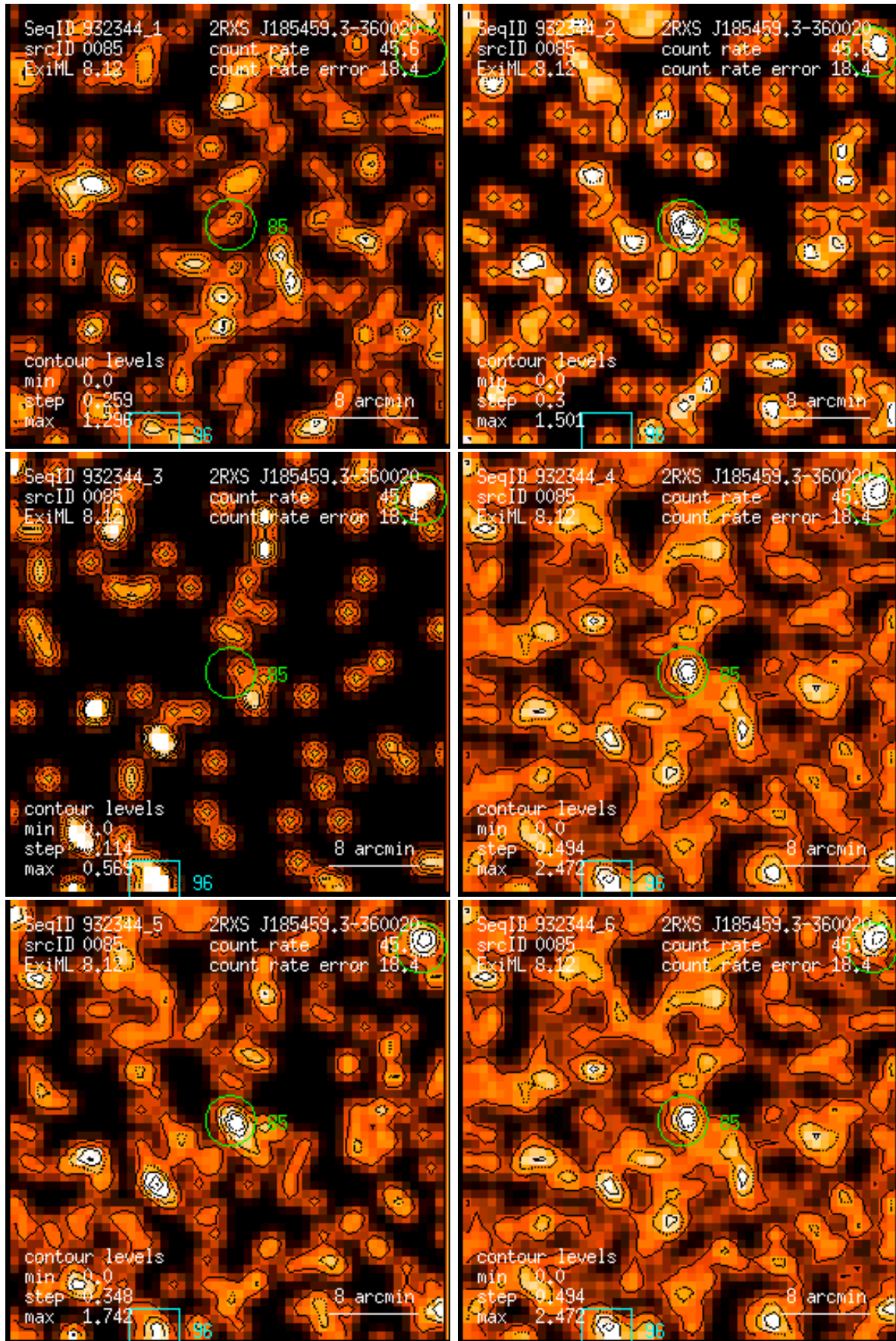
Figure 85: RASS 932344: detection 0085: band rate images, Gaussian filter: (1) PSPC channels 11 – 41, (2) 52 – 90, (3) 91 – 201, (4) 11 – 235, (5) 52 – 201, (6) 11 – 201. Broad band rates in counts/ks. Band rate contour levels in counts/ks/arcmin 2 .
