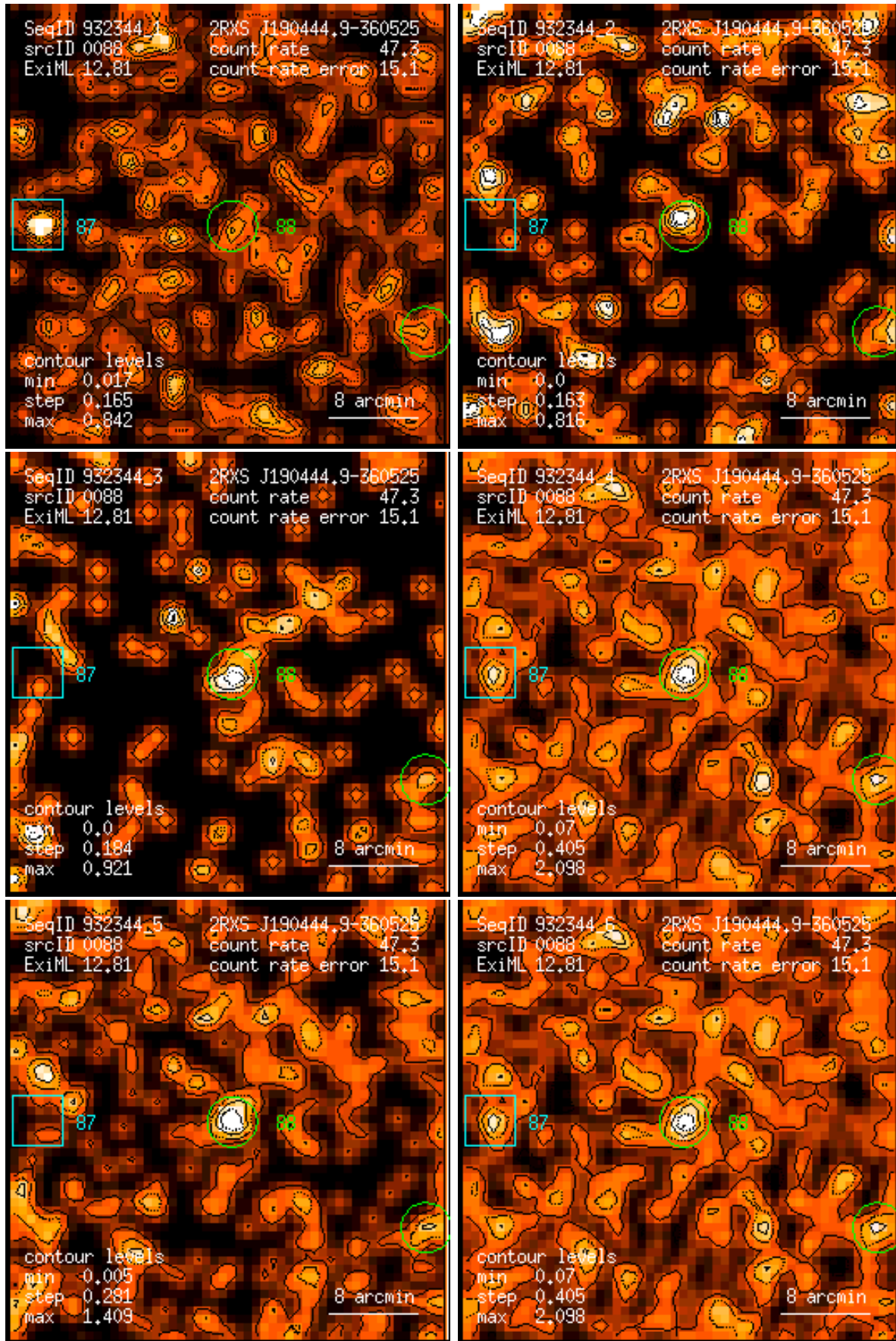
Figure 88: RASS 932344: detection 0088: band rate images, Gaussian filter: (1) PSPC channels 11 – 41, (2) 52 – 90, (3) 91 – 201, (4) 11 – 235, (5) 52 – 201, (6) 11 – 201. Broad band rates in counts/ks. Band rate contour levels in counts/ks/arcmin 2 .
