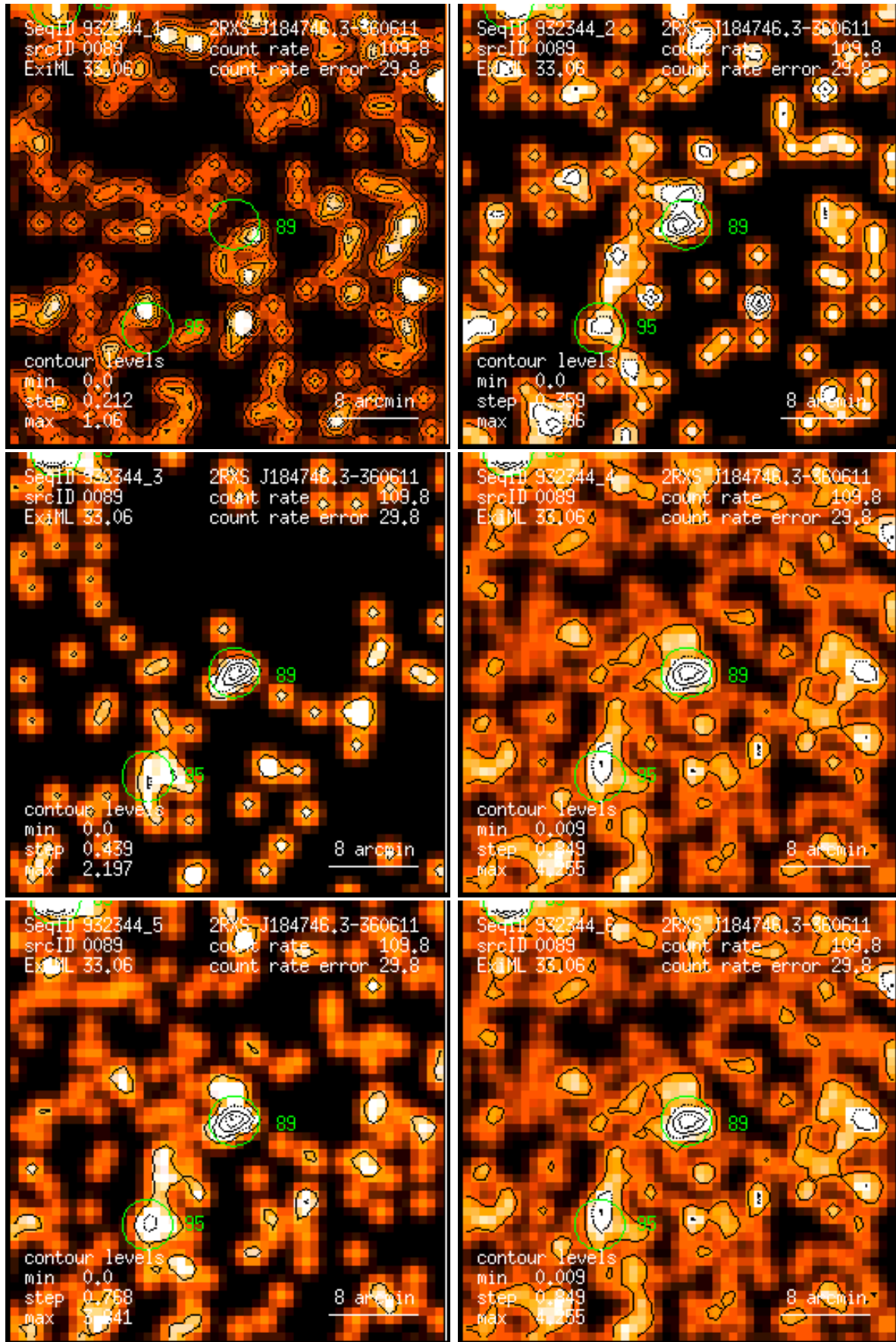
Figure 89: RASS 932344: detection 0089: band rate images, Gaussian filter: (1) PSPC channels 11 – 41, (2) 52 – 90, (3) 91 – 201, (4) 11 – 235, (5) 52 – 201, (6) 11 – 201. Broad band rates in counts/ks. Band rate contour levels in counts/ks/arcmin 2 .
