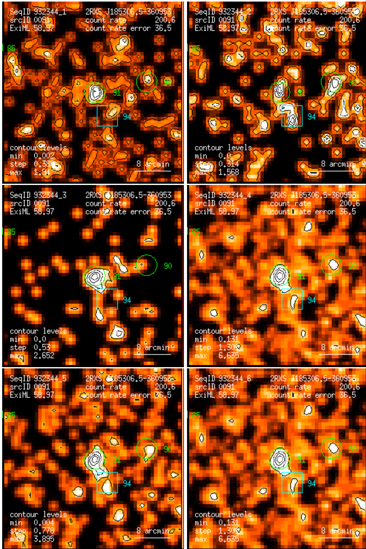
Figure 91: RASS 932344: detection 0091: band rate images, Gaussian filter: (1) PSPC channels 11 – 41, (2) 52 – 90, (3) 91 – 201, (4) 11 – 235, (5) 52 – 201, (6) 11 – 201. Broad band rates in counts/ks. Band rate contour levels in counts/ks/arcmin 2 .
