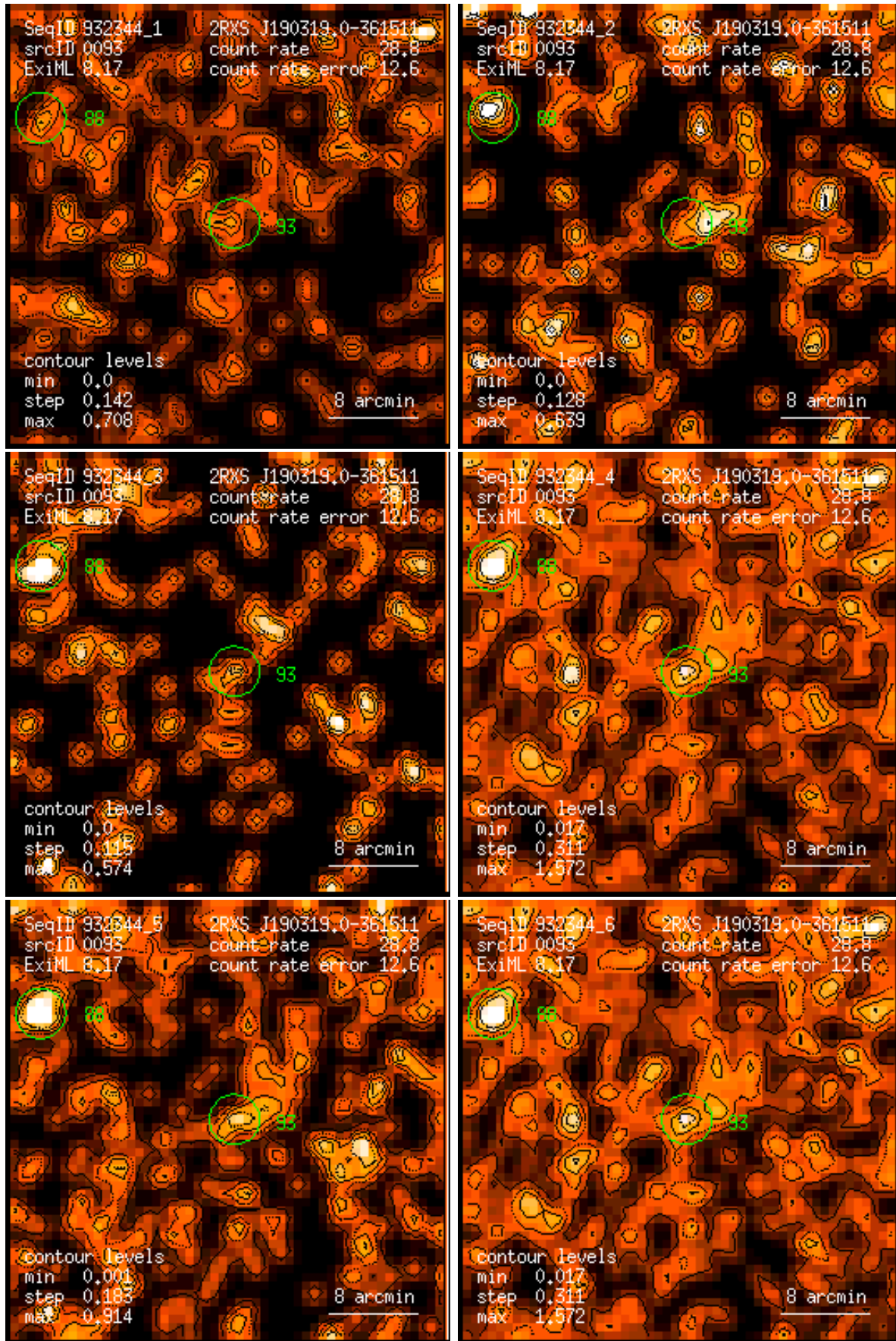
Figure 93: RASS 932344: detection 0093: band rate images, Gaussian filter: (1) PSPC channels 11 – 41, (2) 52 – 90, (3) 91 – 201, (4) 11 – 235, (5) 52 – 201, (6) 11 – 201. Broad band rates in counts/ks. Band rate contour levels in counts/ks/arcmin 2 .
