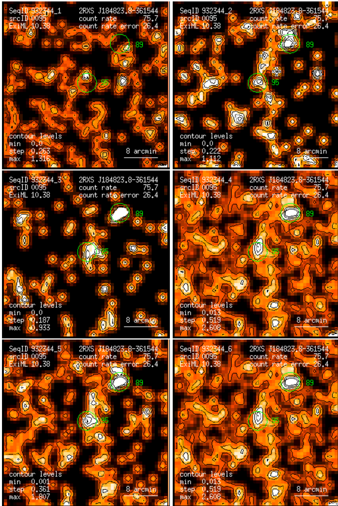
Figure 95: RASS 932344: detection 0095: band rate images, Gaussian filter: (1) PSPC channels 11 – 41, (2) 52 – 90, (3) 91 – 201, (4) 11 – 235, (5) 52 – 201, (6) 11 – 201. Broad band rates in counts/ks. Band rate contour levels in counts/ks/arcmin 2 .
