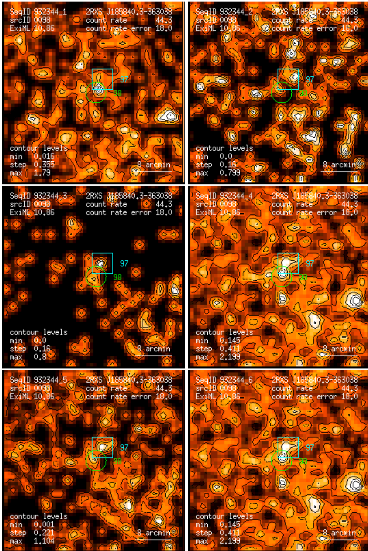
Figure 98: RASS 932344: detection 0098: band rate images, Gaussian filter: (1) PSPC channels 11 – 41, (2) 52 – 90, (3) 91 – 201, (4) 11 – 235, (5) 52 – 201, (6) 11 – 201. Broad band rates in counts/ks. Band rate contour levels in counts/ks/arcmin 2 .
