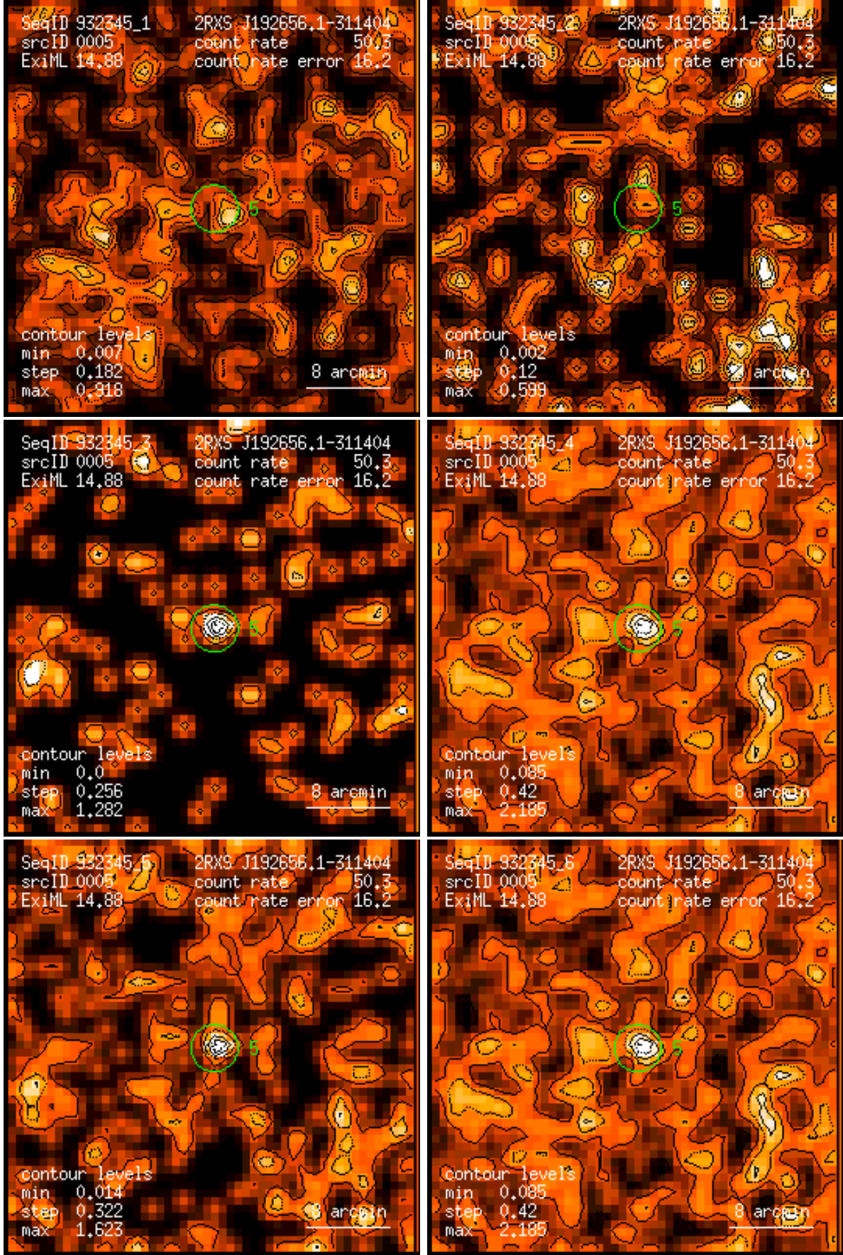
Figure 5: RASS 932345: detection 0005: band rate images, Gaussian filter: (1) PSPC channels 11 – 41, (2) 52 – 90, (3) 91 – 201, (4) 11 – 235, (5) 52 – 201, (6) 11 – 201. Broad band rates in counts/ks. Band rate contour levels in counts/ks/arcmin 2 .
