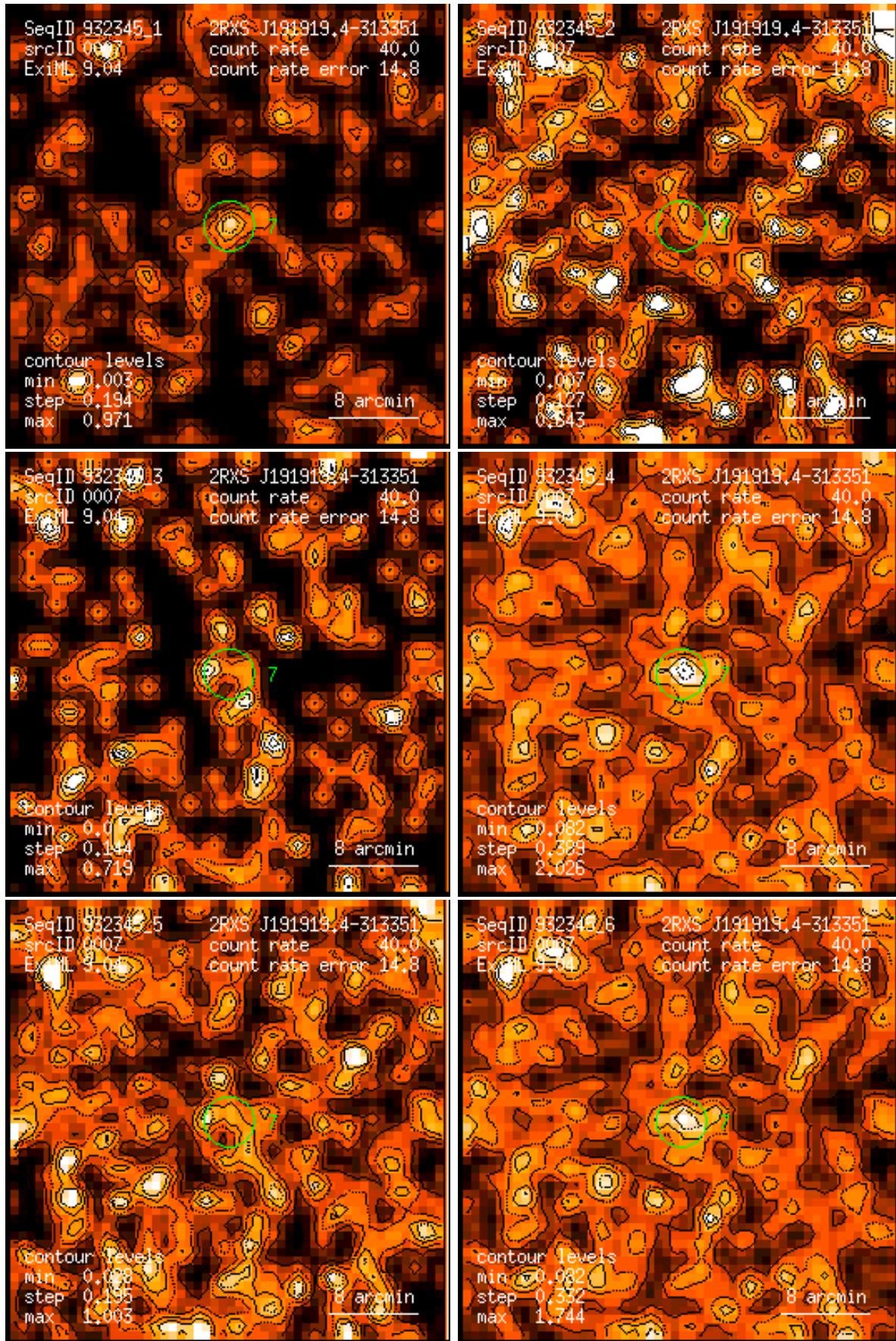
Figure 7: RASS 932345: detection 0007: band rate images, Gaussian filter: (1) PSPC channels 11 – 41, (2) 52 – 90, (3) 91 – 201, (4) 11 – 235, (5) 52 – 201, (6) 11 – 201. Broad band rates in counts/ks. Band rate contour levels in counts/ks/arcmin 2 .
