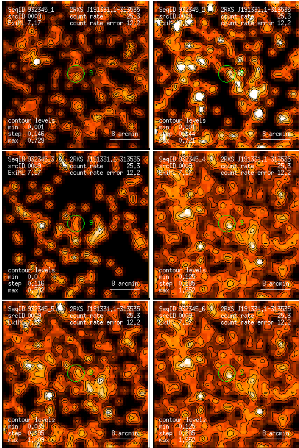
Figure 9: RASS 932345: detection 0009: band rate images, Gaussian filter: (1) PSPC channels 11 – 41, (2) 52 – 90, (3) 91 – 201, (4) 11 – 235, (5) 52 – 201, (6) 11 – 201. Broad band rates in counts/ks. Band rate contour levels in counts/ks/arcmin 2 .
