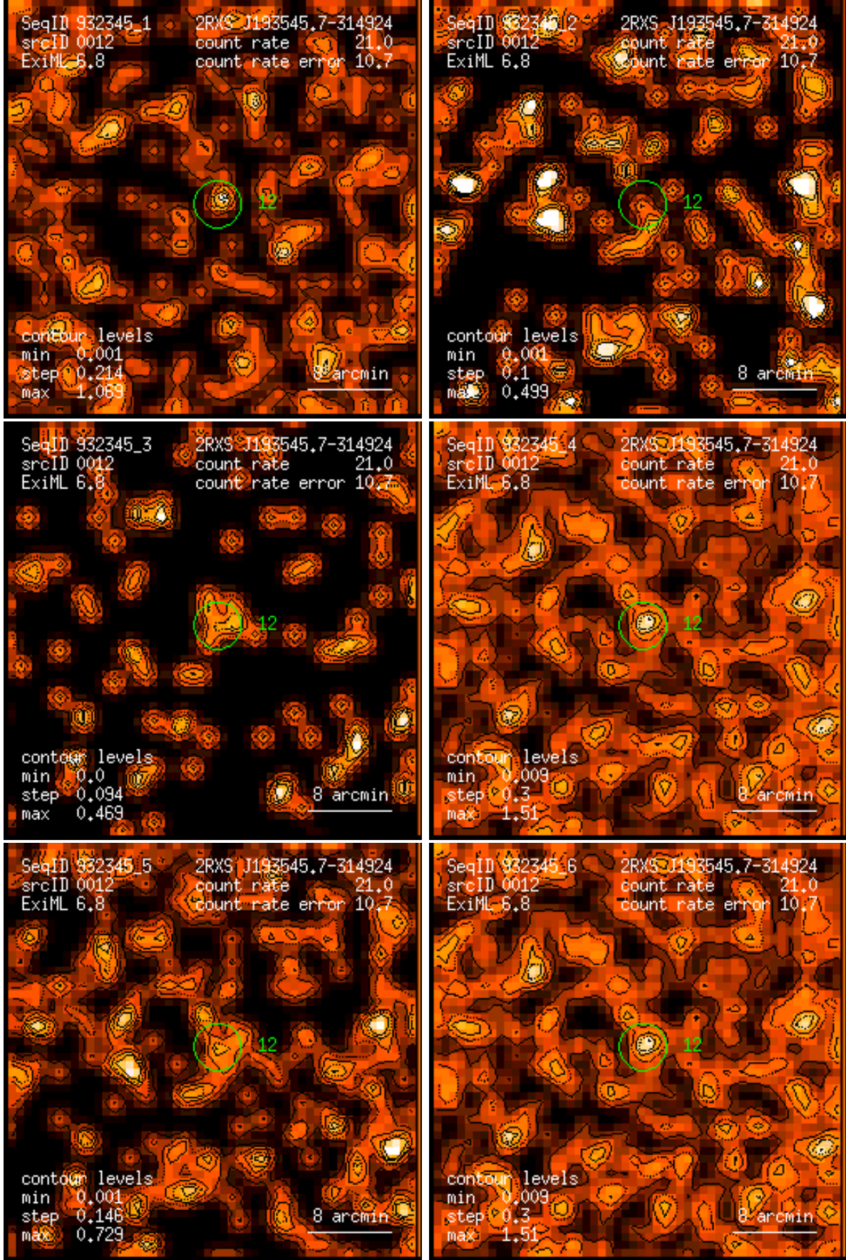
Figure 12: RASS 932345: detection 0012: band rate images, Gaussian filter: (1) PSPC channels 11 – 41, (2) 52 – 90, (3) 91 – 201, (4) 11 – 235, (5) 52 – 201, (6) 11 – 201. Broad band rates in counts/ks. Band rate contour levels in counts/ks/arcmin 2 .
