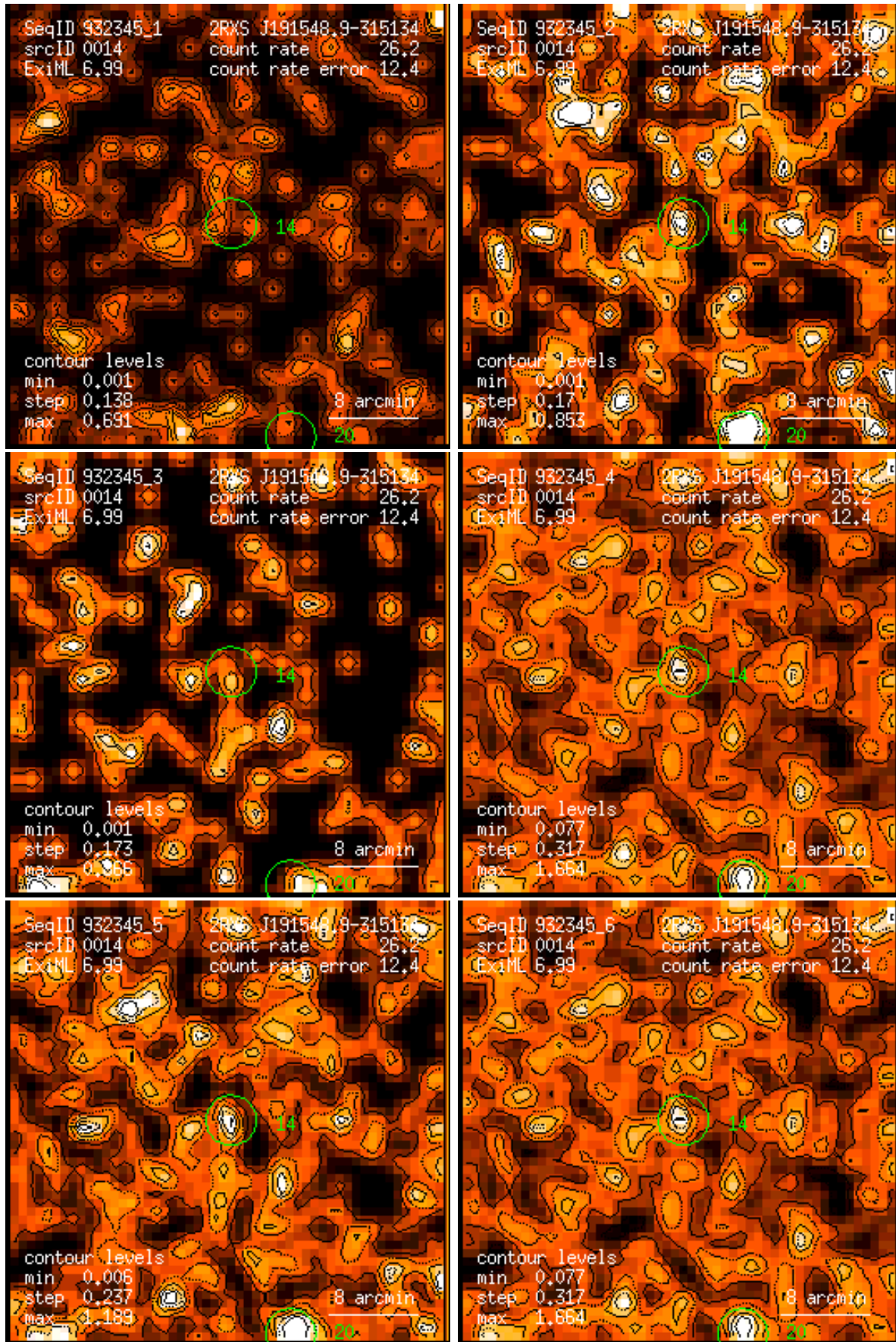
Figure 14: RASS 932345: detection 0014: band rate images, Gaussian filter: (1) PSPC channels 11 – 41, (2) 52 – 90, (3) 91 – 201, (4) 11 – 235, (5) 52 – 201, (6) 11 – 201. Broad band rates in counts/ks. Band rate contour levels in counts/ks/arcmin 2 .
